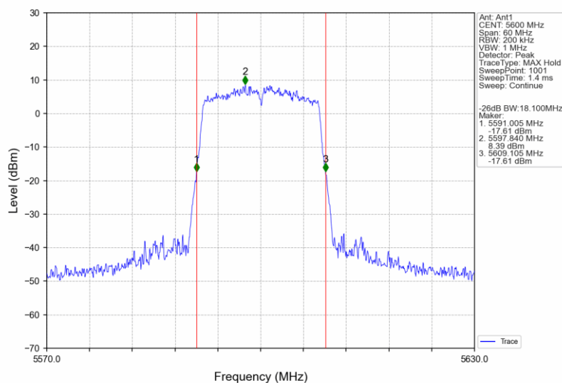
802.11a_MCH_5600MHz_Ant1_NTNV
