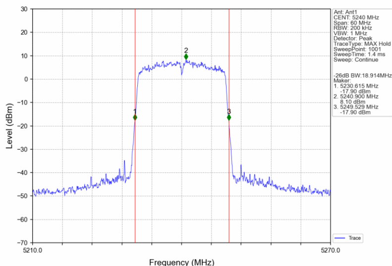
802.11n(HT20)_HCH_5240MHz_Ant1_NTNV
