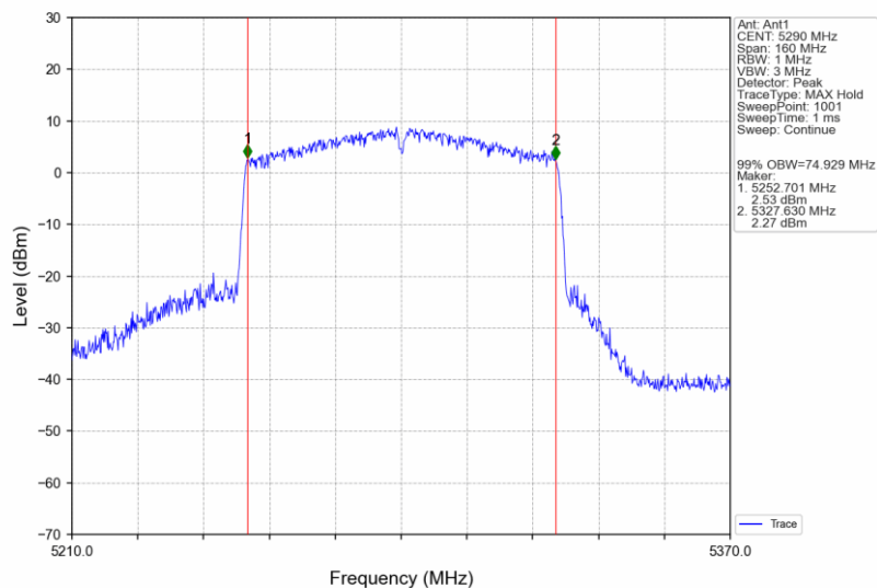
802.11ac(VHT80)_MCH_5290MHz_Ant1_NTNV
