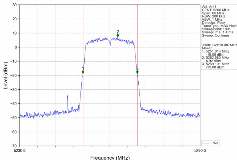
802.11a_LCH_5260MHz_Ant1_NTNV
