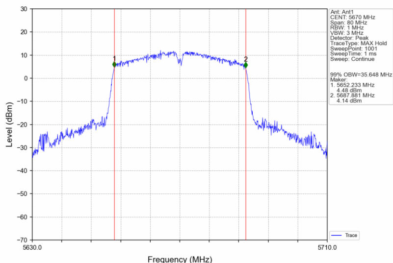
802.11ac(VHT40)_HCH_5670MHz_Ant1_NTNV
