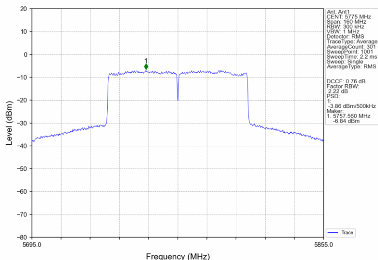
802.11ac(VHT80)_MCH_5775MHz_Ant1_NTNV
