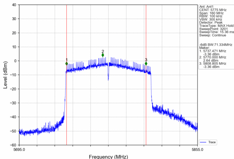
802.11ac(VHT80)_MCH_5775MHz_Ant1_NTNV
