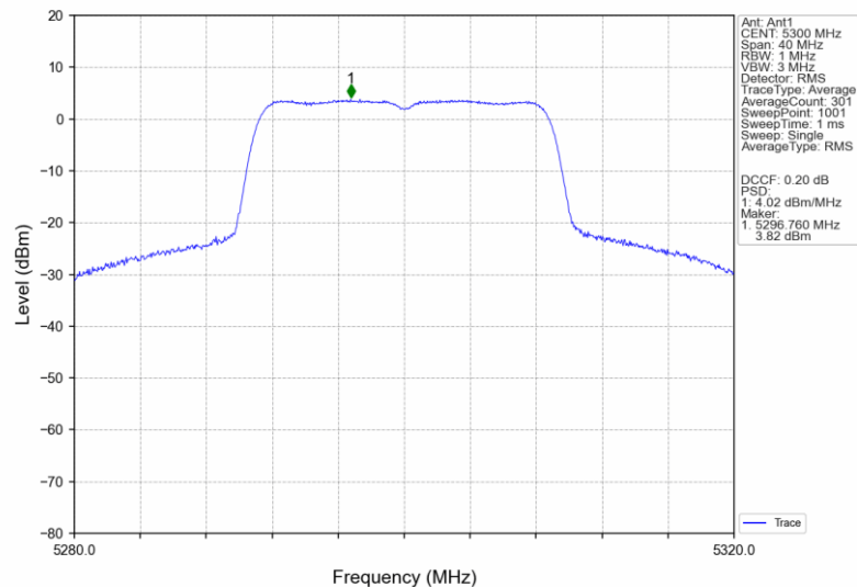
802.11ac(VHT20)_MCH_5300MHz_Ant1_NTNV
