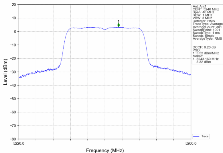
802.11ac(VHT20)_HCH_5240MHz_Ant1_NTNV
