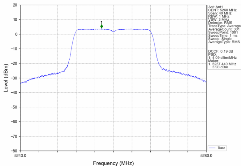
802.11a_LCH_5260MHz_Ant1_NTNV
