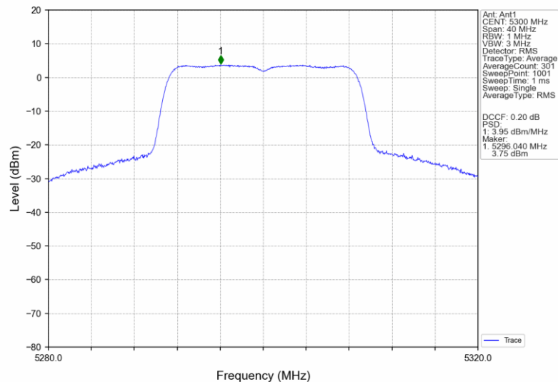
802.11n(HT20)_MCH_5300MHz_Ant1_NTNV
