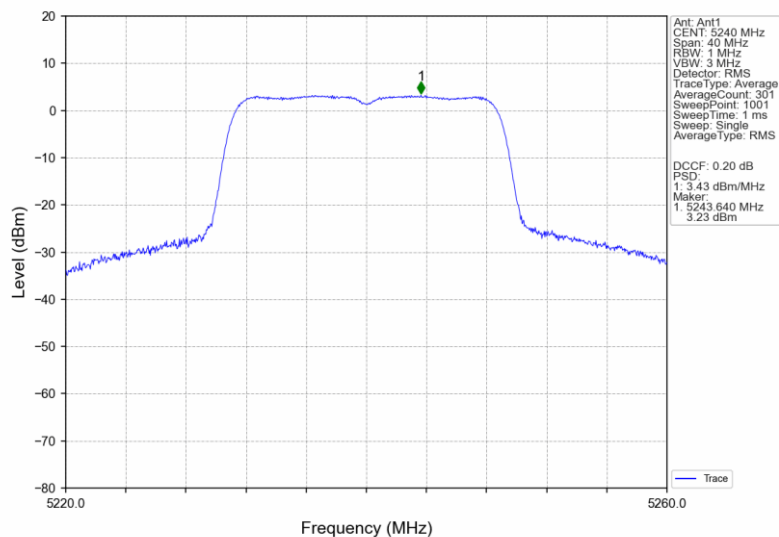
802.11n(HT20)_HCH_5240MHz_Ant1_NTNV
