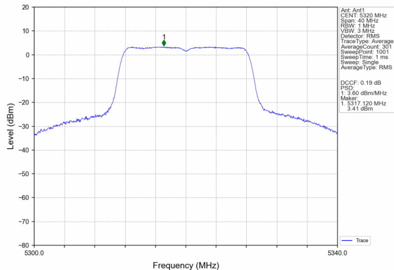
802.11a_HCH_5320MHz_Ant1_NTNV
