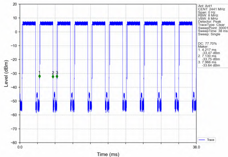
8DPSK_3DH5_MCH_2441MHz_Ant1_NTNV
