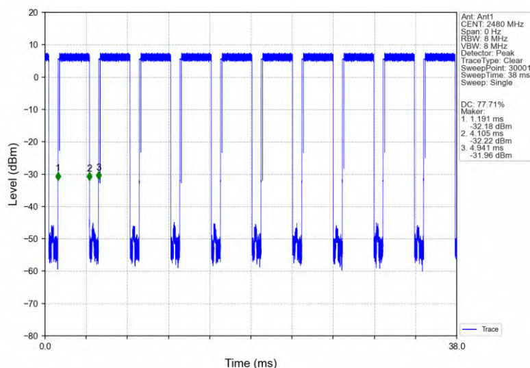
Pi/4DQPSK_2DH5_HCH_2480MHz_Ant1_NTNV
