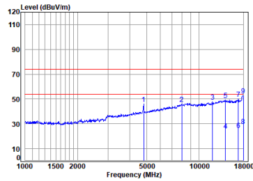
BT_DH5_TX_CH_00_Horizontal
