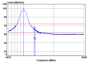
BT_DH5_TX_CH_78_Vertical
