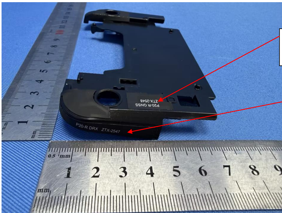
GNSS antenna
