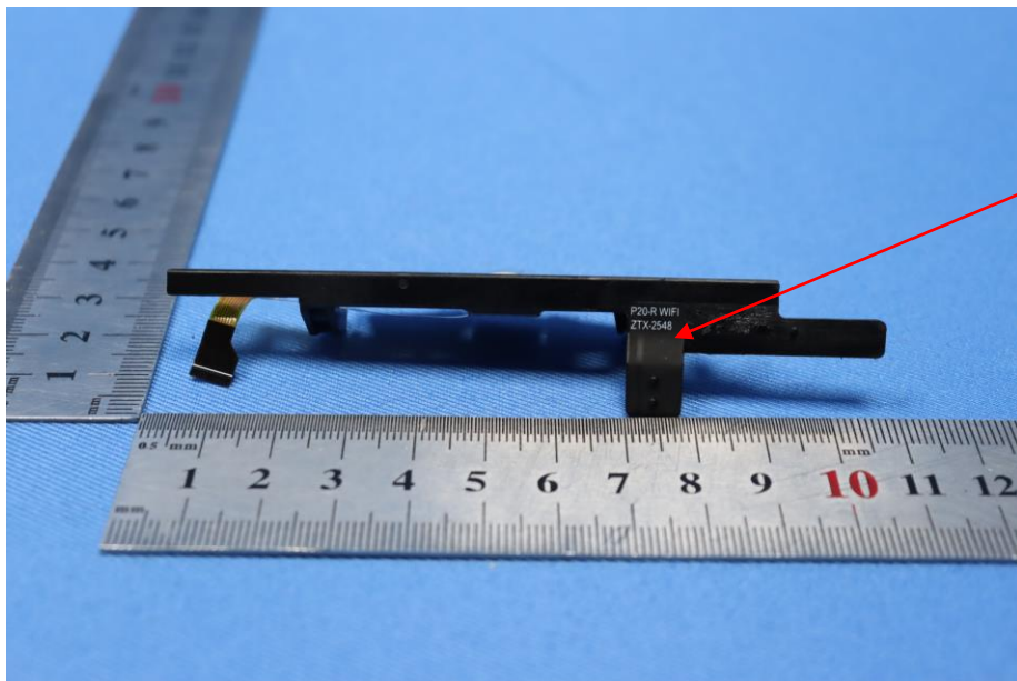
BT/Wi-Fi antenna
