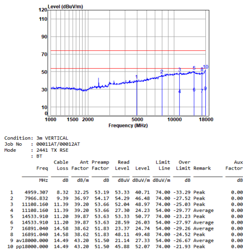
BT_DH5_TX_CH_39_Vertical
