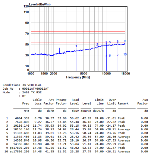
BT_DH5_TX_CH_00_Vertical
