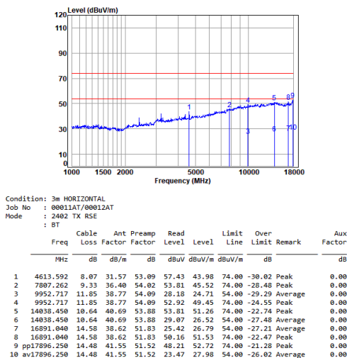
BT_DH5_TX_CH_00_Horizontal
