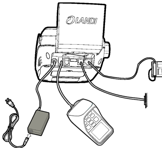
Figure 5.4 Connection Example
