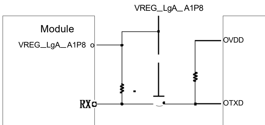
Figure 4.13 : Schematic diagram of RX level conversion
