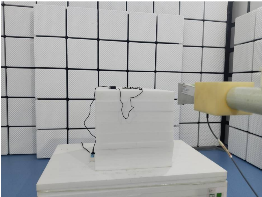
RSE - Front View (18 G-40 GHz)
