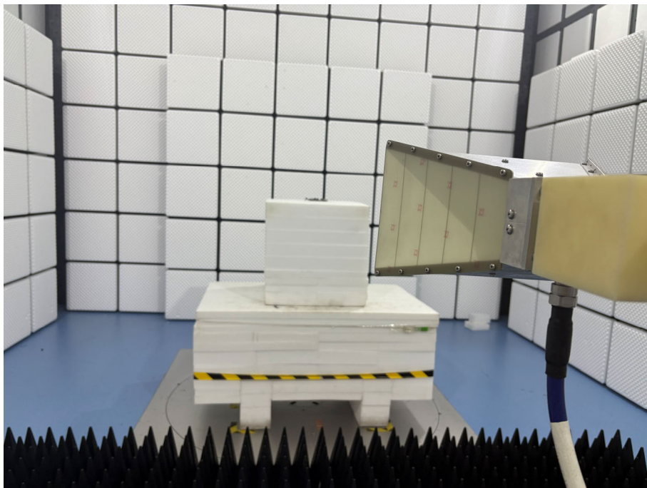
RSE - Front View (1 G-18 GHz)
