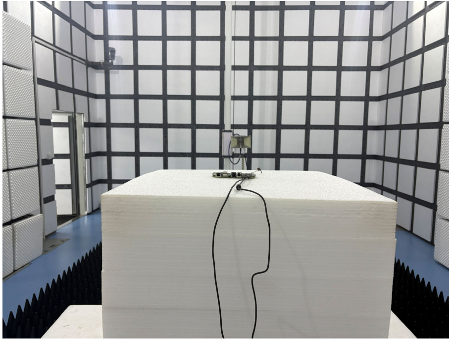
RSE - Front View (Above 18 G)
