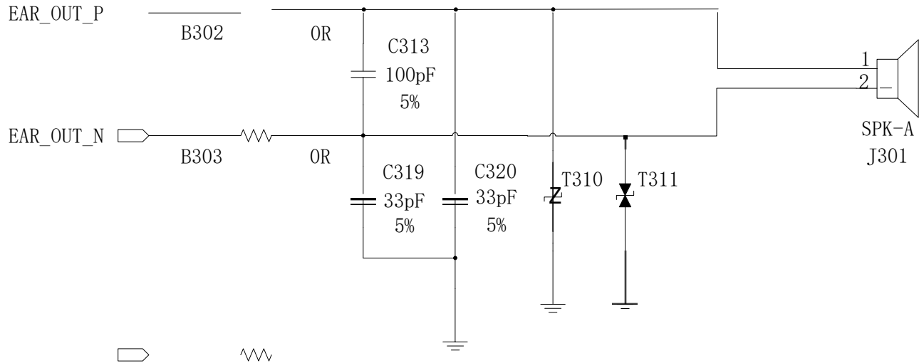
Figure 4.18: Receiver reference circuit
