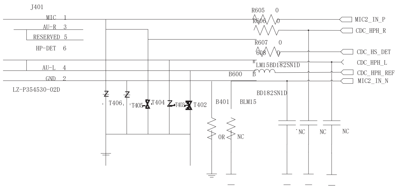
Figure 4.21: Headphone jack circuit
