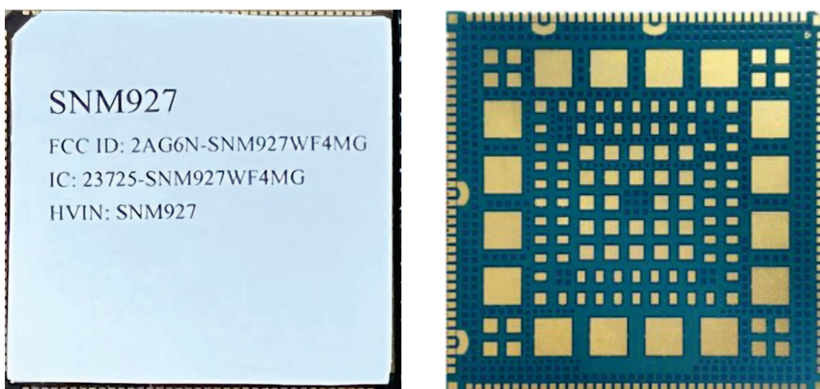
Figure 6.1: Top view and bottom view of the module
