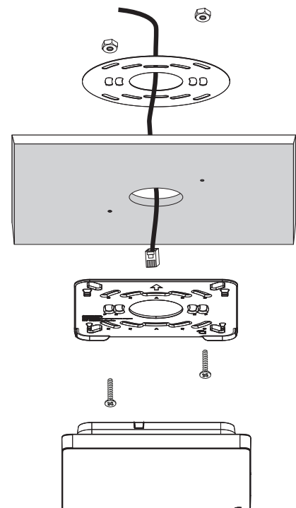
Figure 8. Ceiling Tile Mounting
