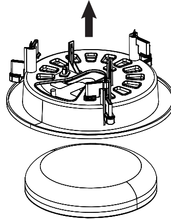
Ⓒ In-Ceiling Mount
