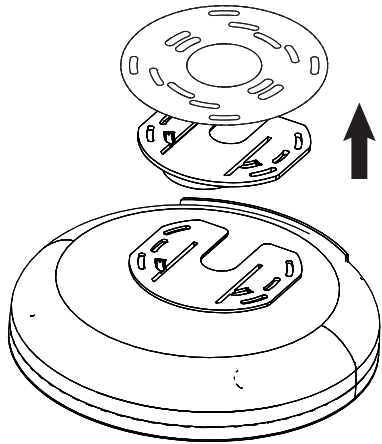
Ⓐ Ceiling Mount
