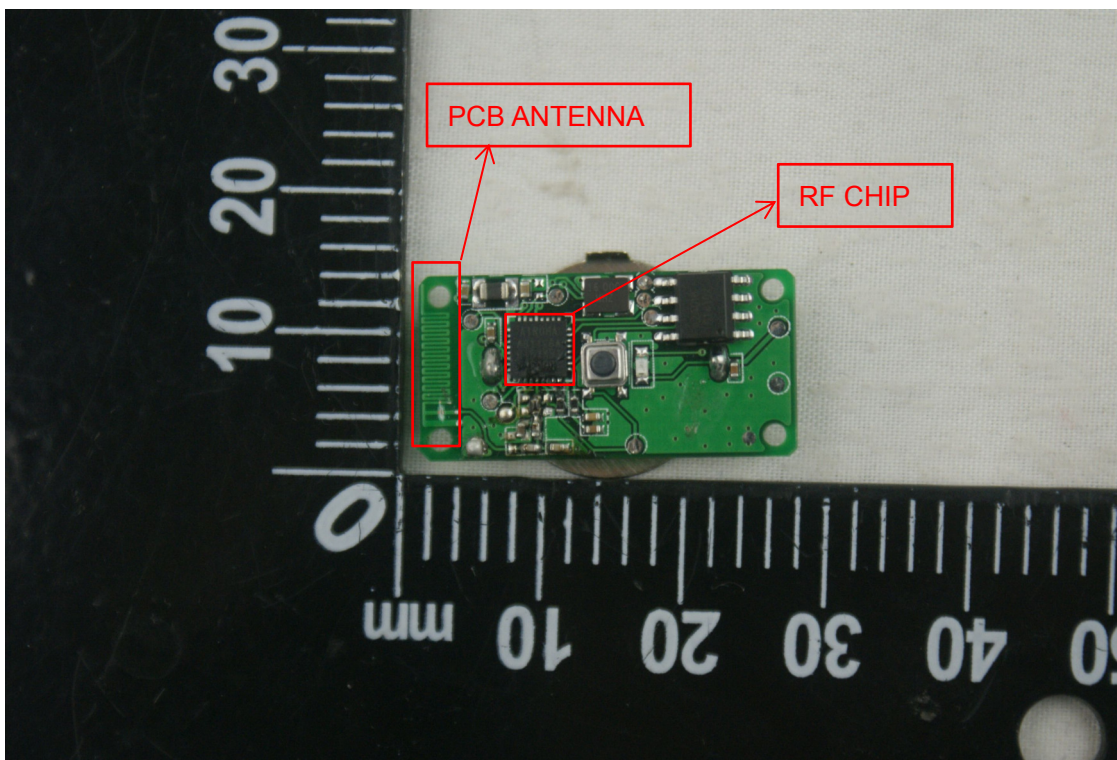
MAIN BOARD VIEW 1
