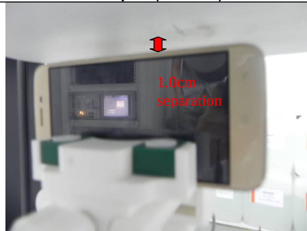
Hotspot(RIGHT EDGE)
