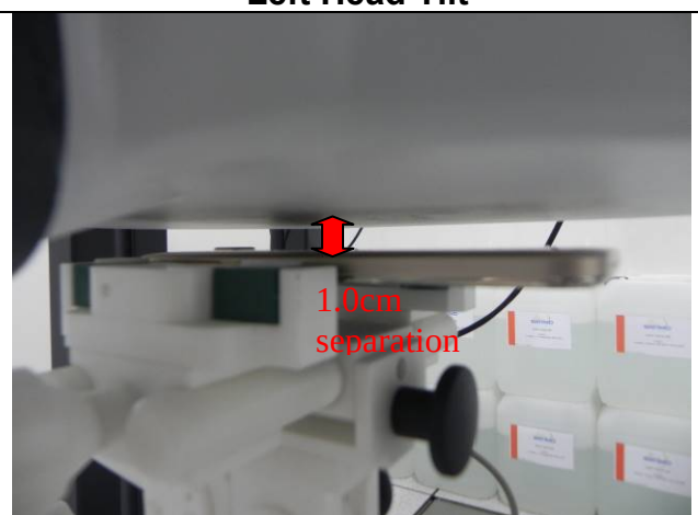
Body-Worn(LCD Down)
