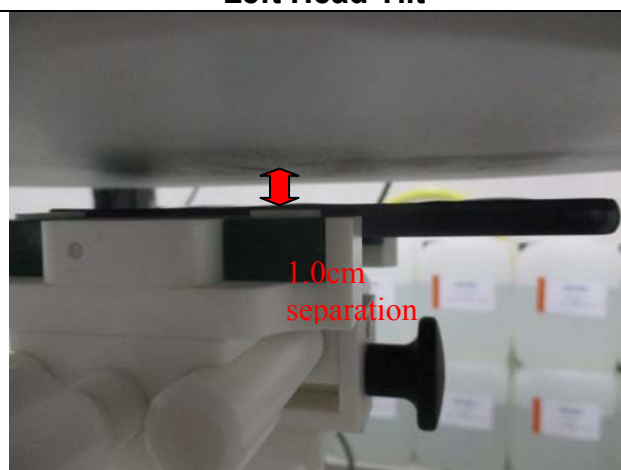
Body-Worn(LCD Down)
