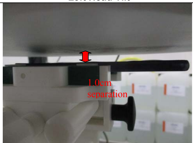
Body-Worn(LCD Down)
