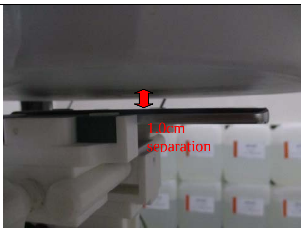
Hotspot(LCD Down)
