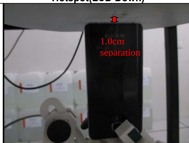
Hotspot(BOTTOM EDGE)
