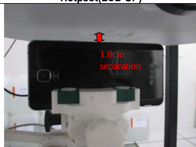
Hotspot(LEFT EDGE)
