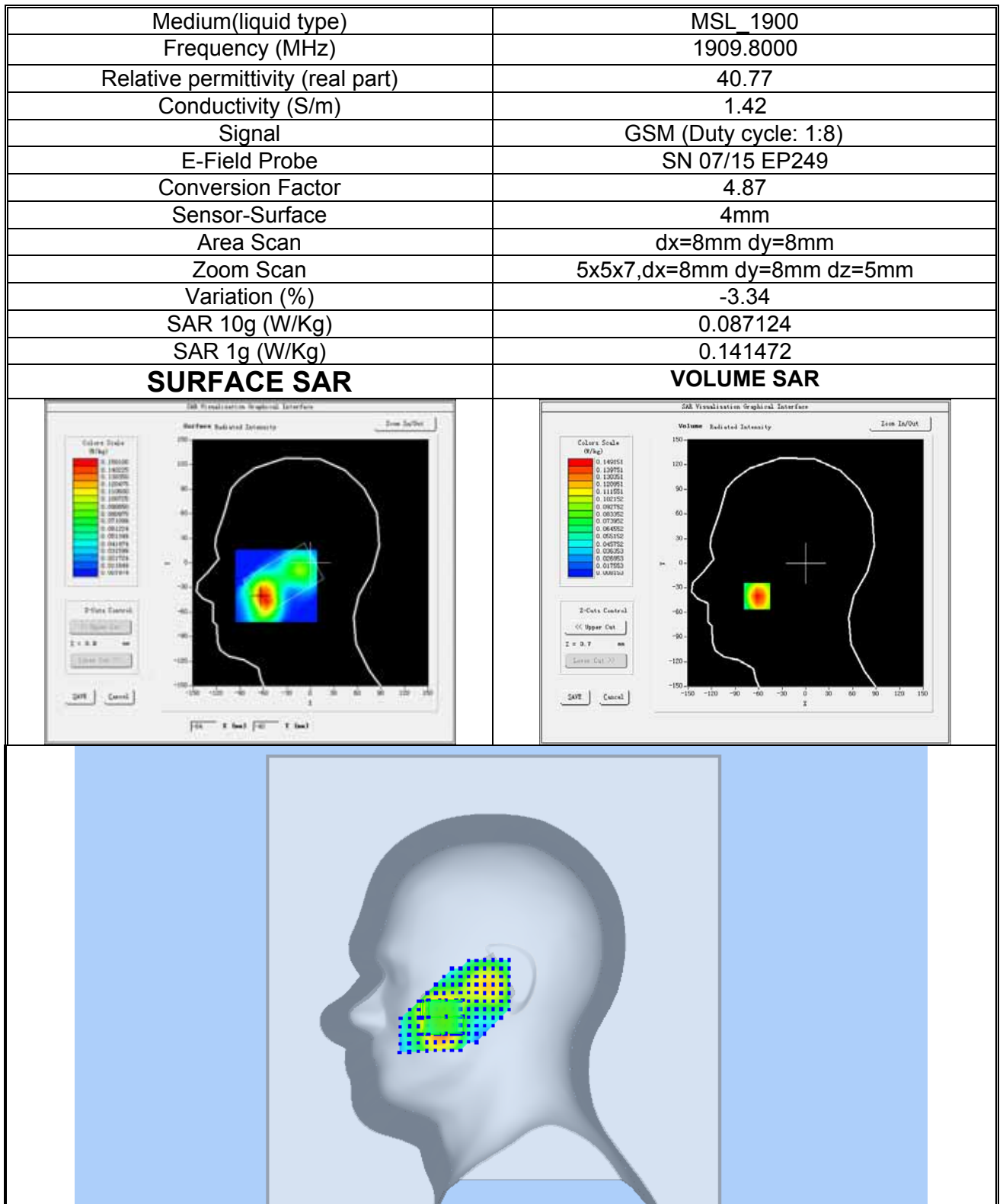
Plot 10: GSM1900, High channel (Right Head, Tilt) Product Description: Mobile Phone Test Date: 2018-05-31
