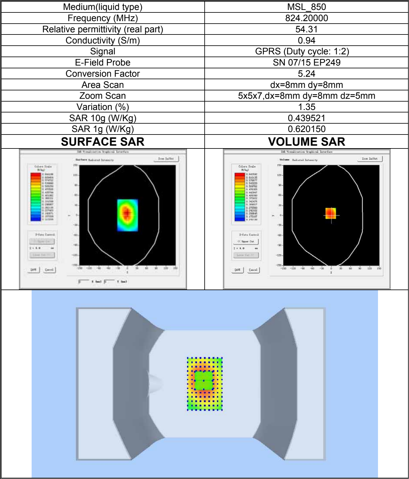
Plot 7: GPRS850MHz, Low channel(Body-worn, Right edge) Product Description: Mobile Phone Test Date: 2018-06-04
