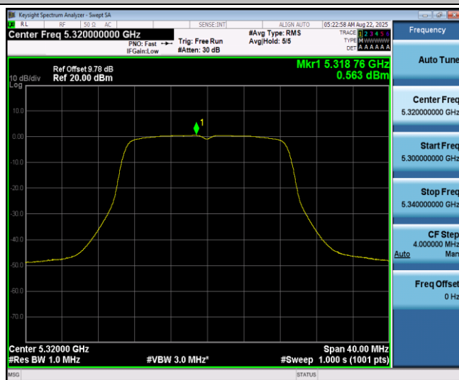
11N20SISO_Ant1_5320
