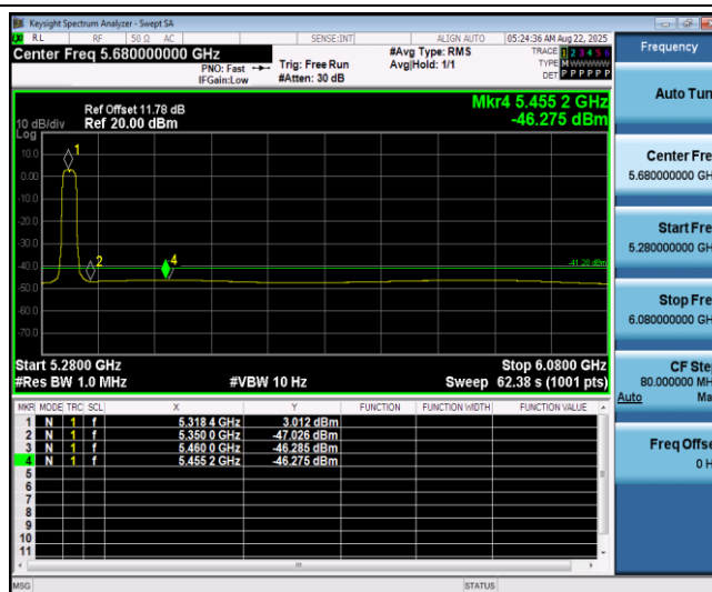
11N20SISO_Ant1_High_5320_Peak
