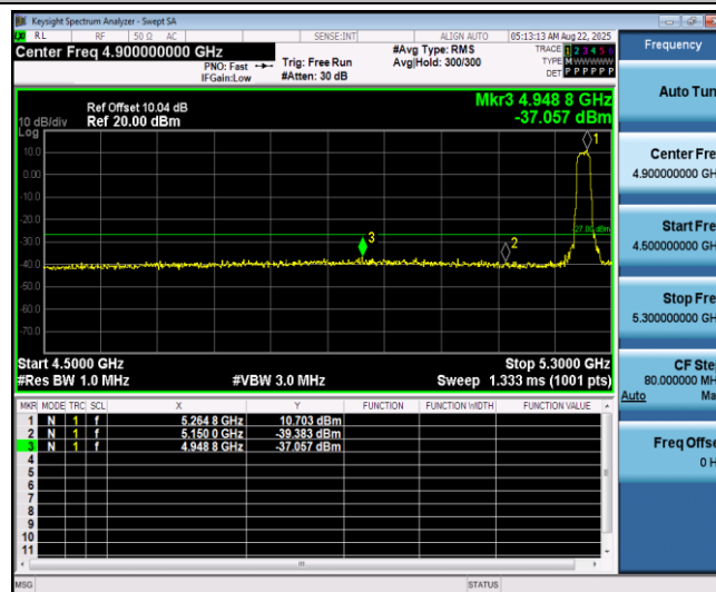
11N20SISO_Ant1_Low_5260
