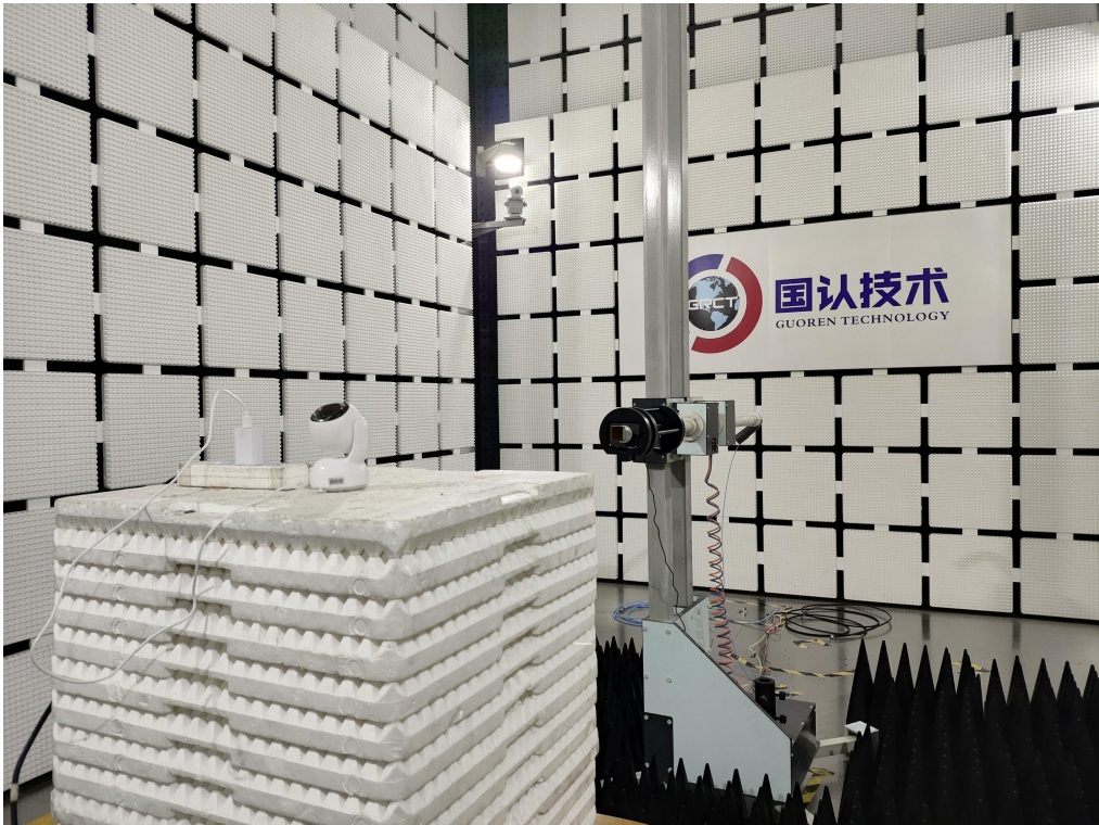
Radiated Emission (Above 40 GHz)
