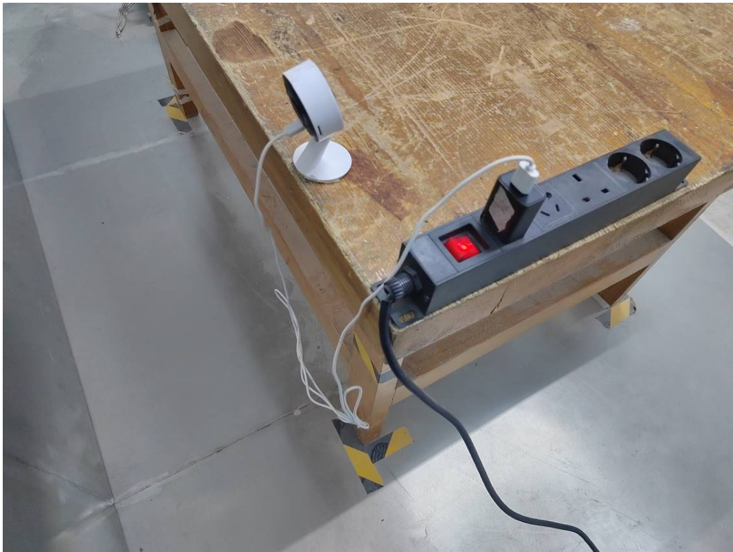
Conducted Emissions Side View - Mini 16S- Adapter 2#
