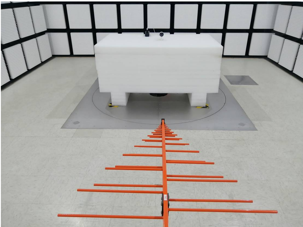
Radiated Emissions Below1G rear View Mini 16S- Adapter 2#
