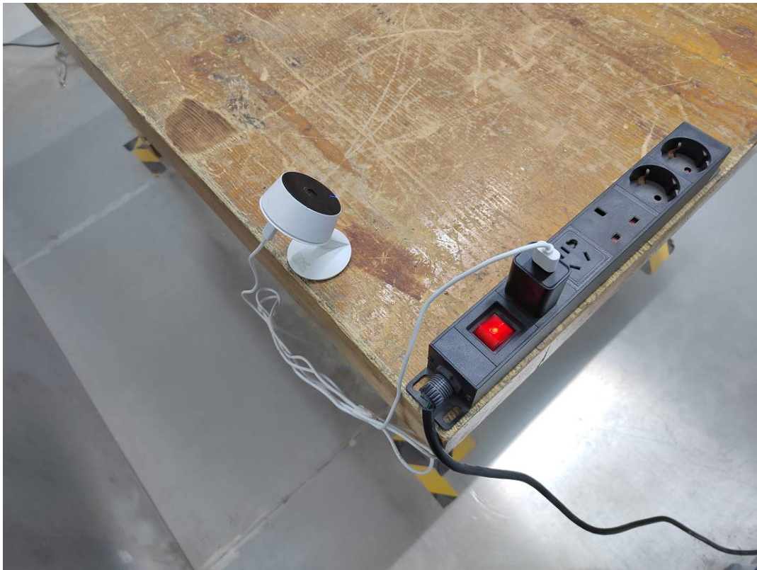
Conducted Emissions Side View - Mini 12S- Adapter 2#
