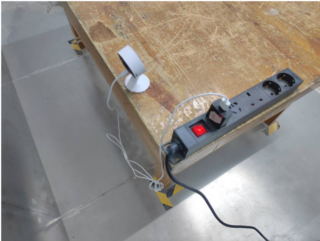
Conducted Emissions Side View - Mini 16S- Adapter 1#
