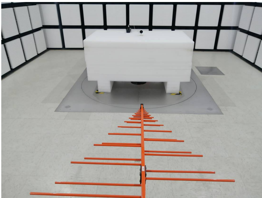
Radiated Emissions Below1G rear View Mini 12S- Adapter 2#
