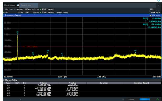
802.11ax40 on Channel 06
