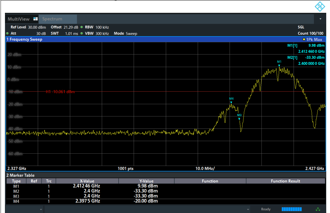
Band Edge NVNT b 2412MHz Ant1 Emission
