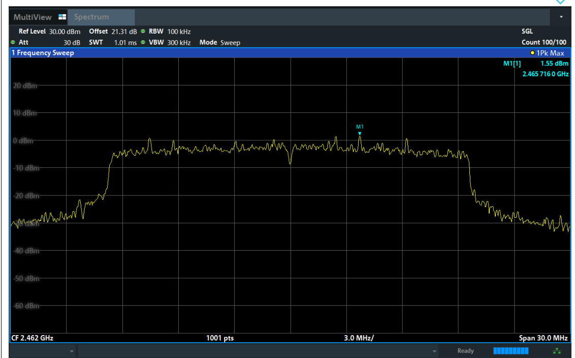
Band Edge NVNT ax20 2462MHz Ant1 Emission
