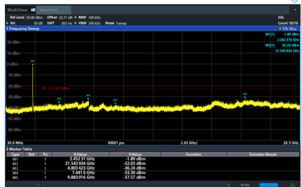
802.11ax40 on Channel 09
