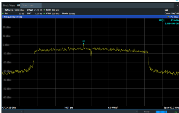
802.11ax40 on Channel 03
