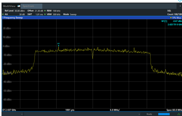
802.11ax40 on Channel 06
