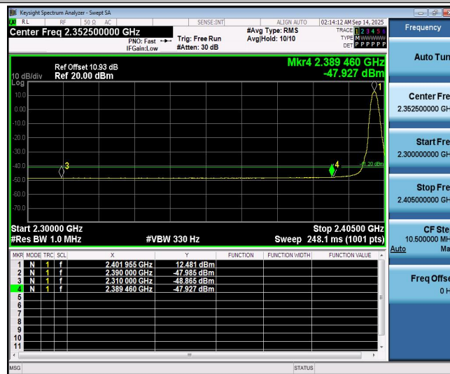
BLE_Ant1_Low_2402_Peak
