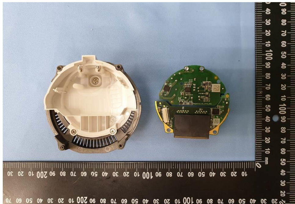
EUT Photo (26)
