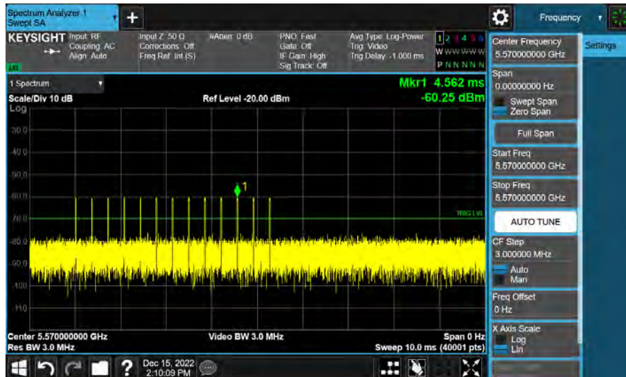
Short Pulse Radar Type 4
