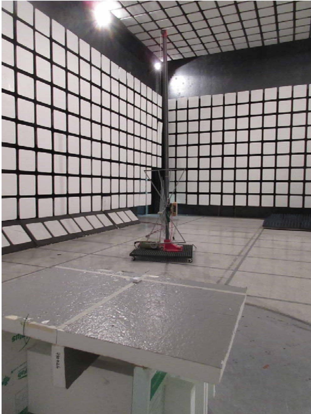
Radiated Emissions at 3 m, 30 – 1000 MHz
