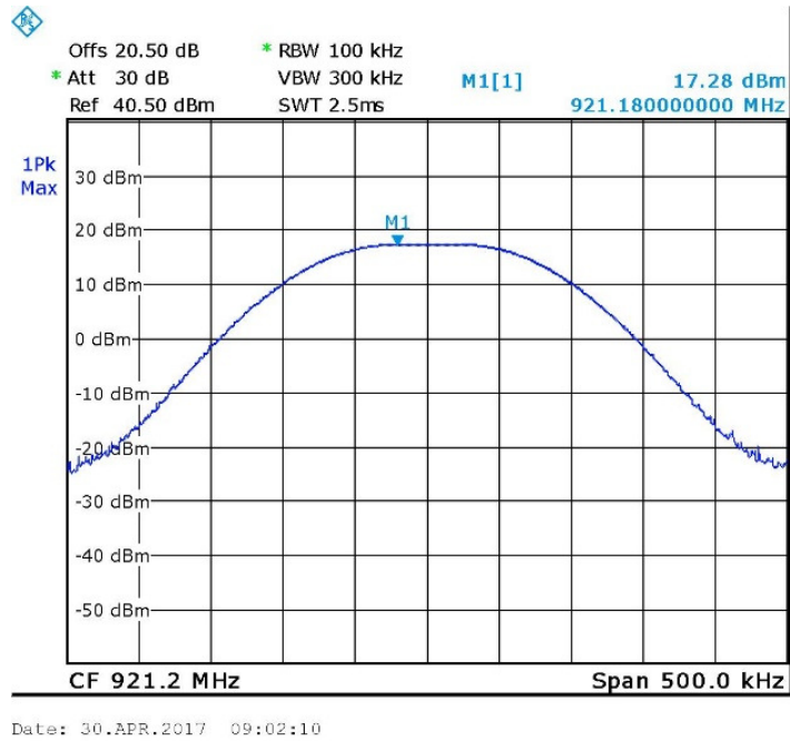
Figure 26 — 921.2 MHz
