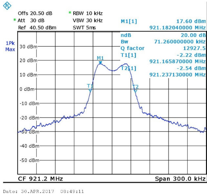
Figure 9. — 921.2 MHz
