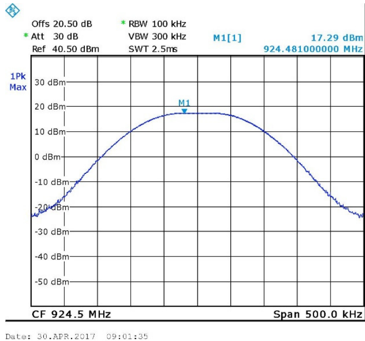
Figure 27 — 924.5 MHz
