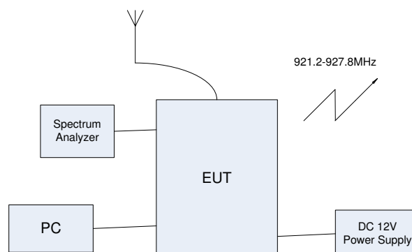
Figure 1. Configuration of Tested System - Radiated
