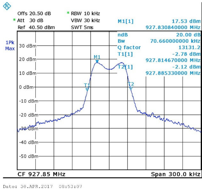
Figure 11. — 927.8 MHz
