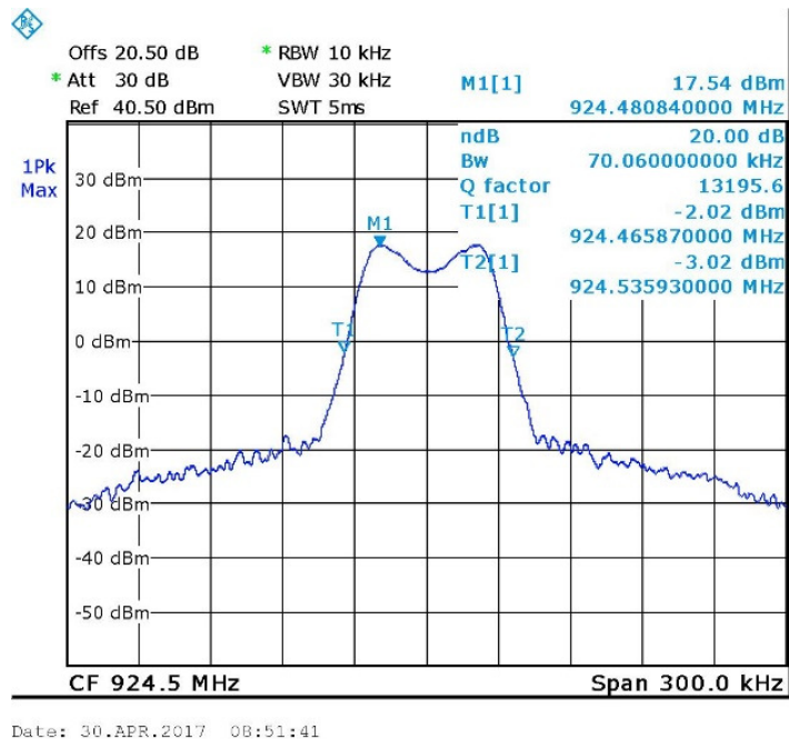
Figure 10. — 924.5 MHz
