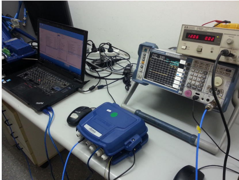
Figure 7. Conducted Tests
