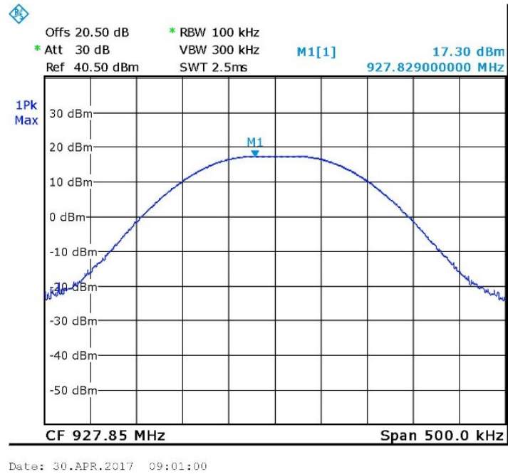
Figure 28 — 927.8 MHz
