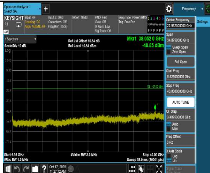
11AC20SISO_Ant2_5825_30~5650
