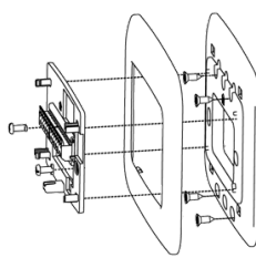
2 gang (4" square) box (wall plate sold separately)
