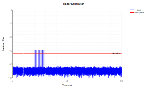
Radar #4
