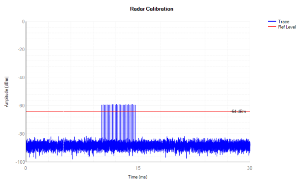
Radar #4
