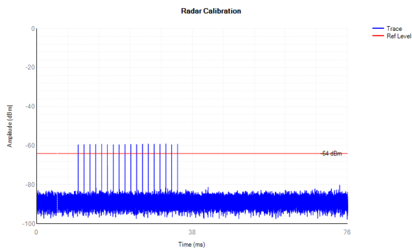
Radar #2
