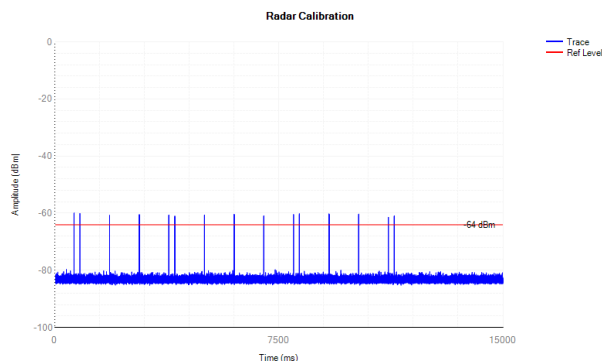
Radar #5
