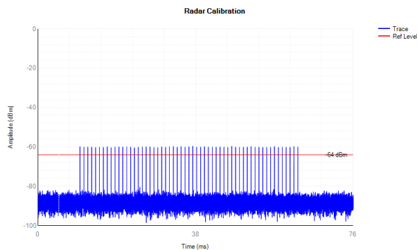
Radar #3
