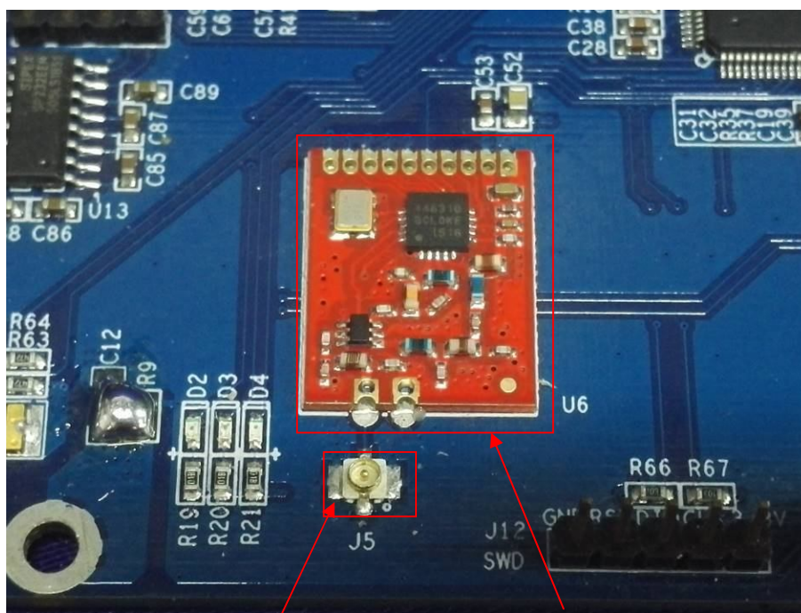
Antenna Port
