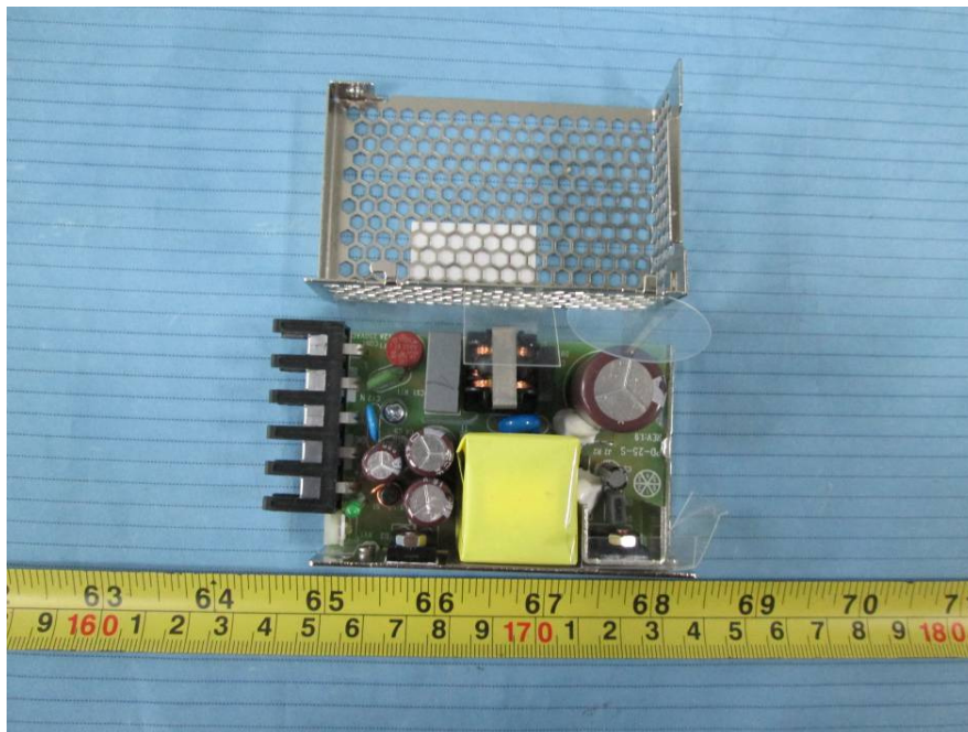
EUT – DC Power Cover off 1 View
