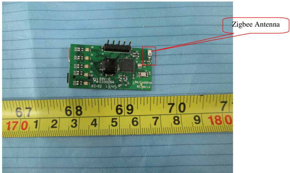
EUT – Zigbee Main Board Top View
