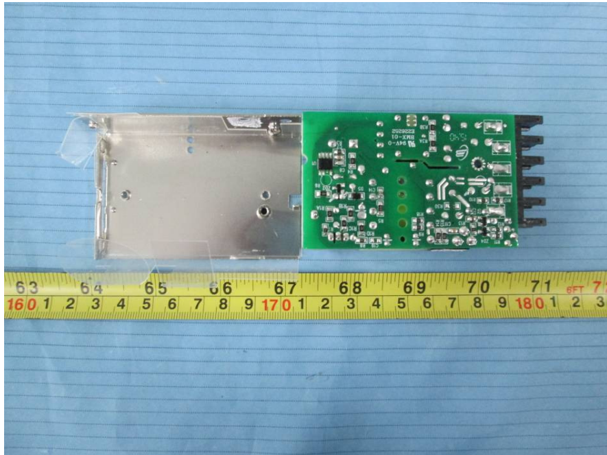
EUT – DC Power Cover off 2 View
