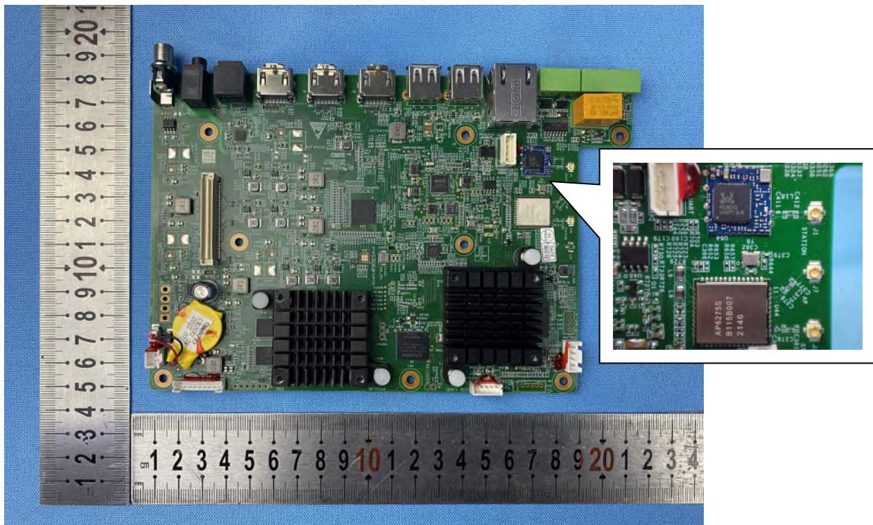
Photo 6: Main Board-upper side
