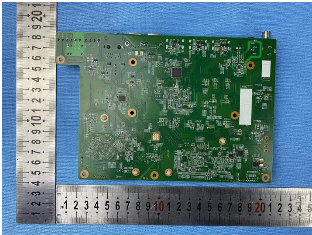
Photo 7: Main Board-bottom side
