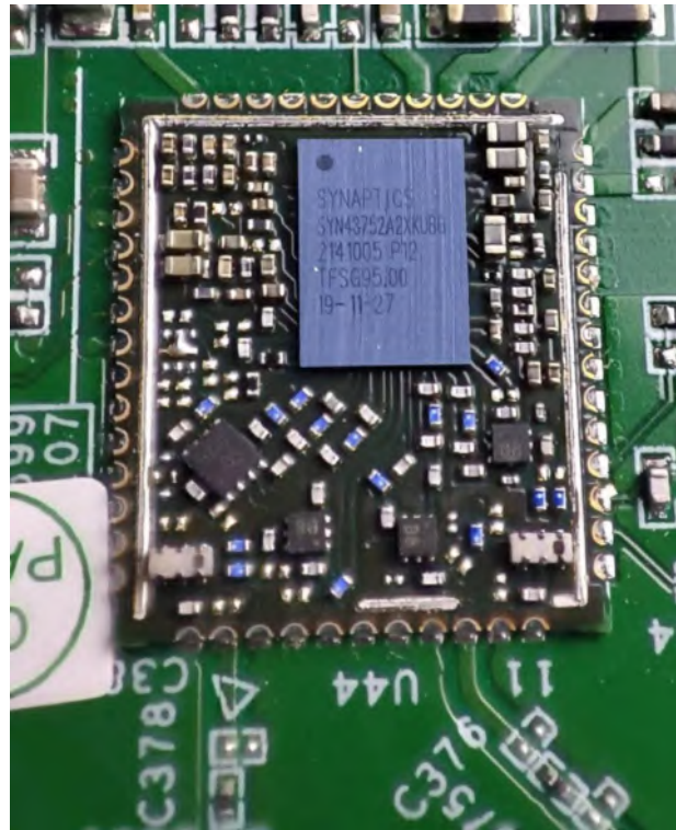
Photo 9: Internal View for WiFi-AP & BT Module
