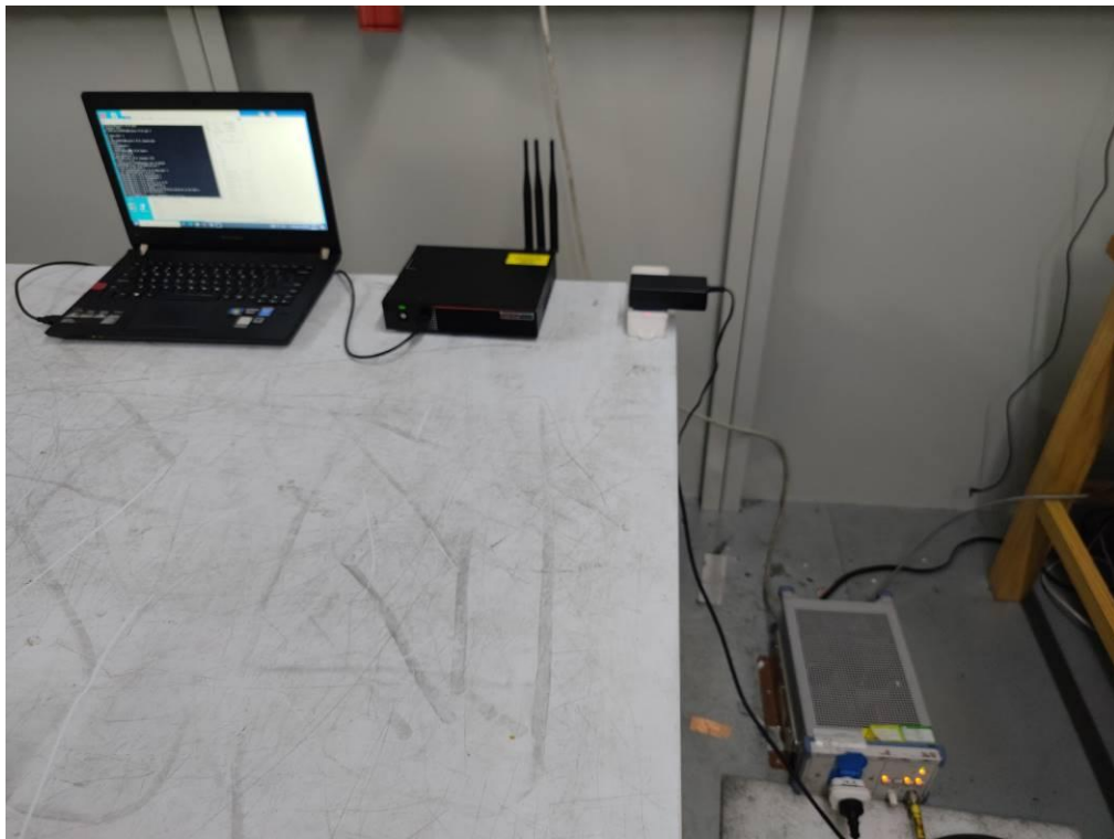
Description: Conducted Emissions Test Setup
