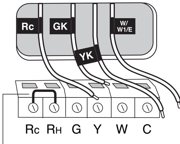
Jumper wire
