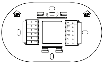
Mounting Plate
