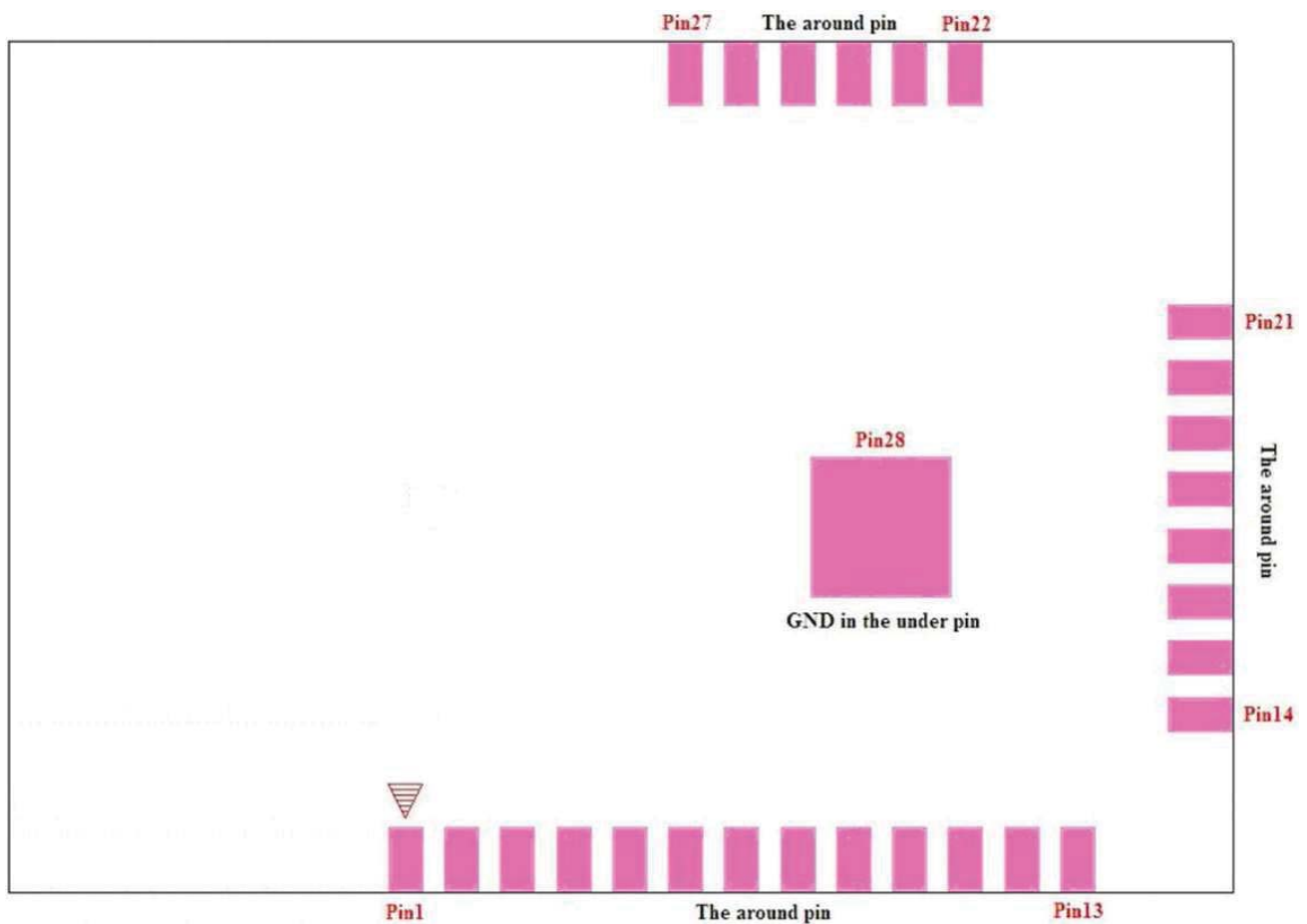
Figure-4 Module Pin Out (Top View)
