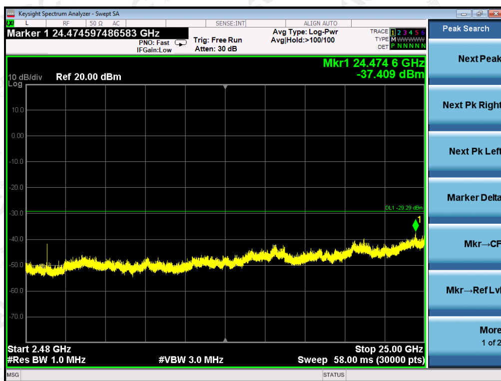
TEST PLOTS OF 802.11g OUT OF BAND EMISSIONS MODULATION IN LOW CHANNEL
