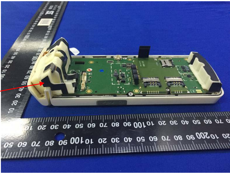
WIFI/BT Antenna
