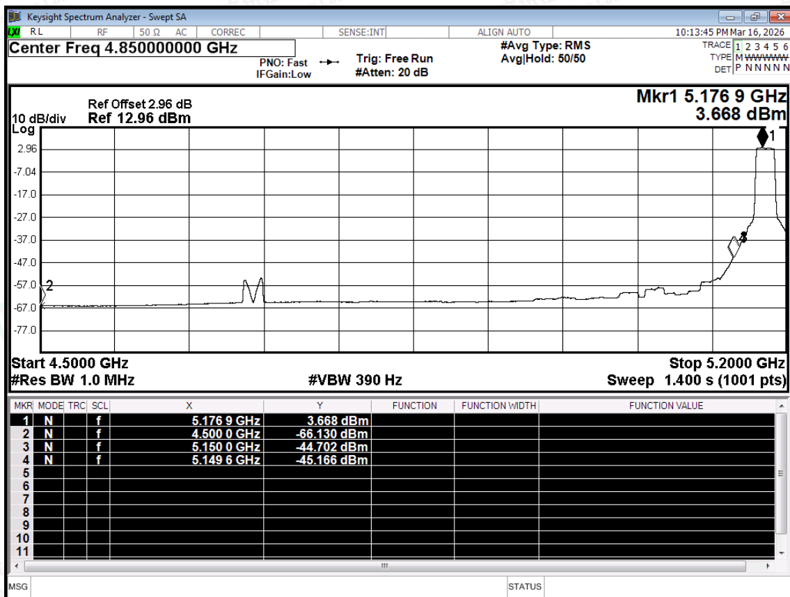
Restrict Band NVNT a 5180MHz Ant1 Average
