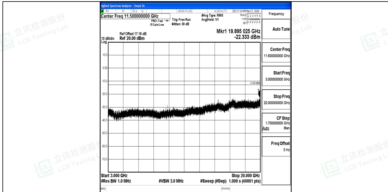
Band2_20MHz_16QAM_18700_1RB#0_3000~20000_3000~20000
