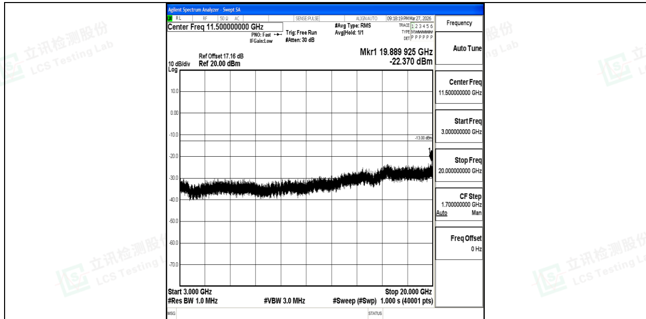
Band2_20MHz_16QAM_18900_1RB#0_3000~20000_3000~20000
