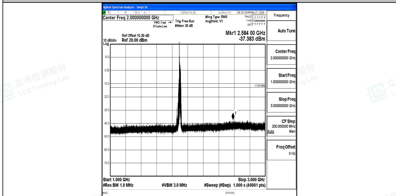
Band2_20MHz_16QAM_19100_1RB#0_1000~3000_1000~3000
