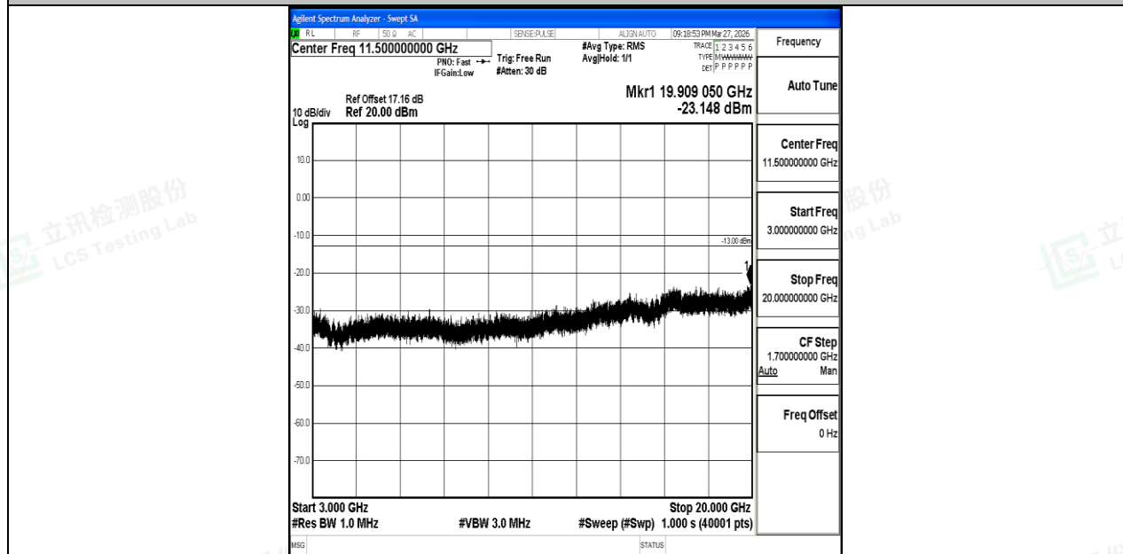
Band2_20MHz_QPSK_19100_1RB#0_3000~20000_3000~20000
