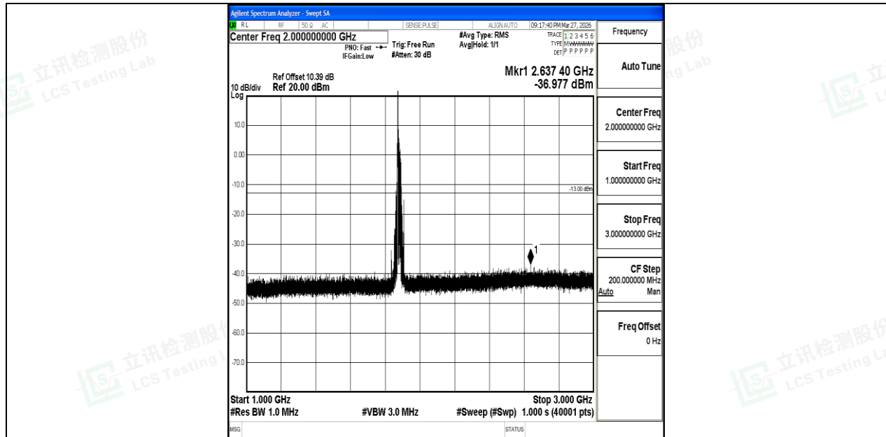
Band2_20MHz_QPSK_18900_1RB#0_1000~3000_1000~3000
