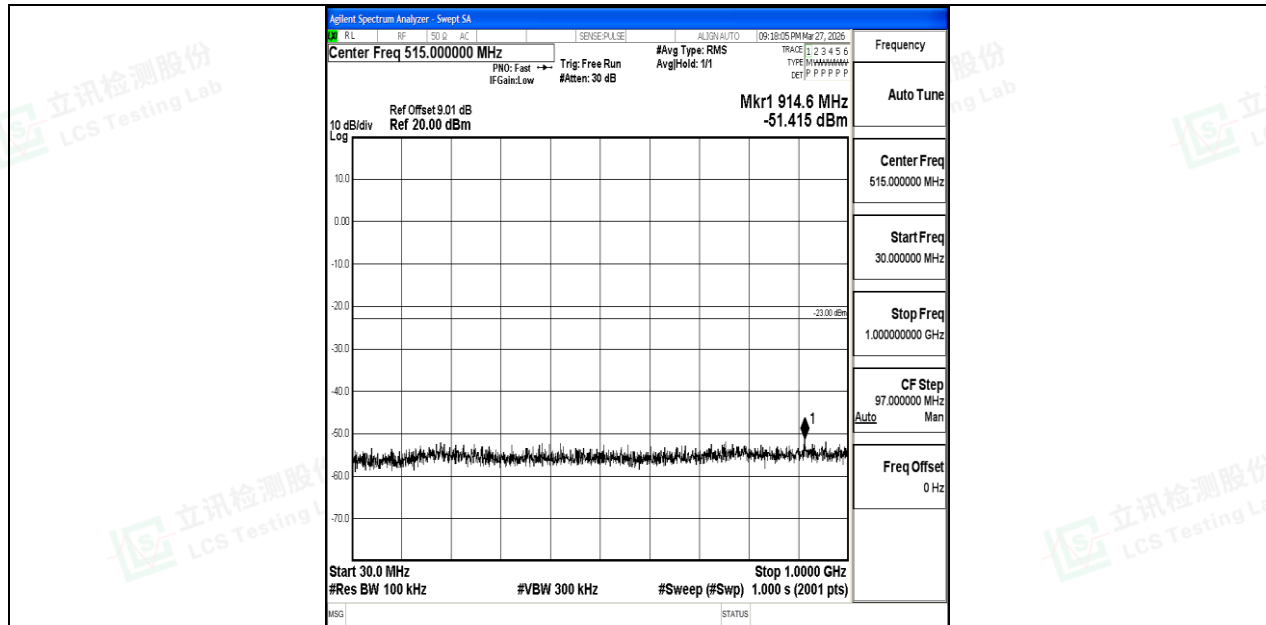
Band2_20MHz_16QAM_18900_1RB#0_30~1000_30~1000
