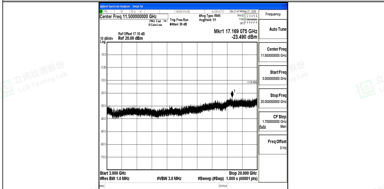
Band2_20MHz_QPSK_18900_1RB#0_3000~20000_3000~20000
