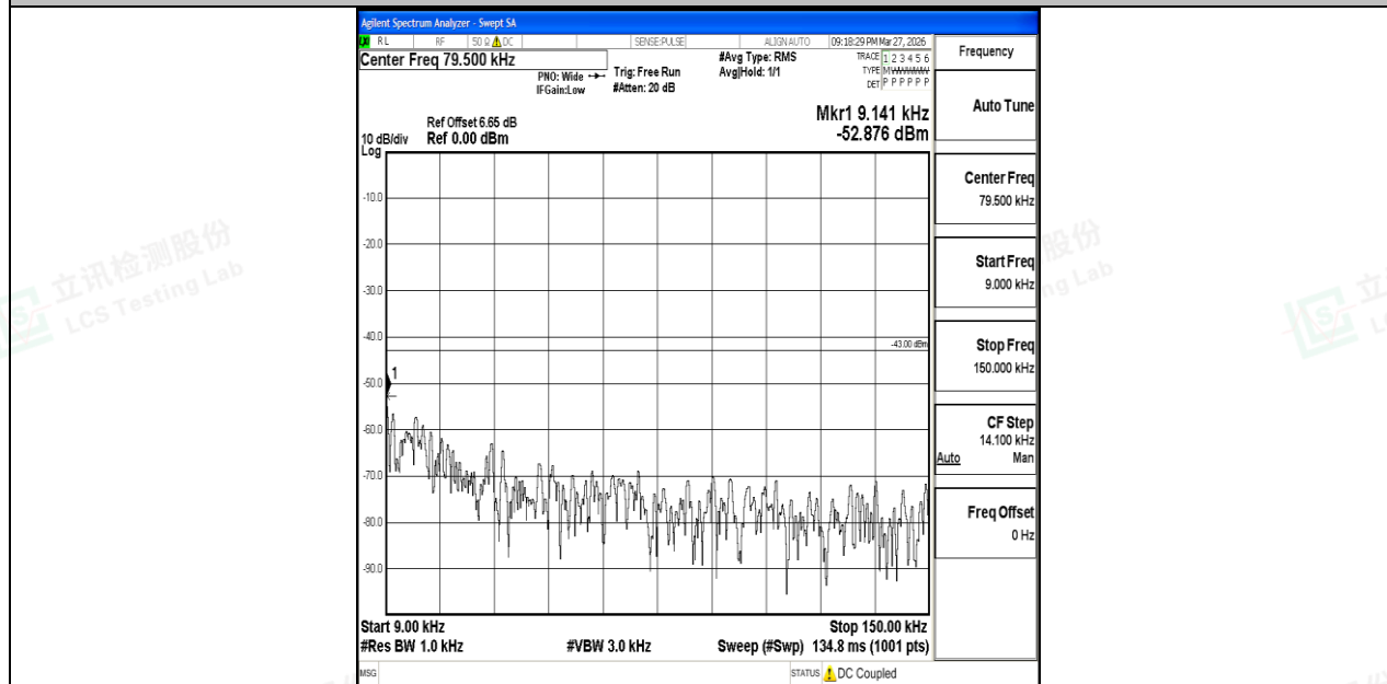
Band2_20MHz_QPSK_19100_1RB#0_0.009~0.15_0.009~0.15
