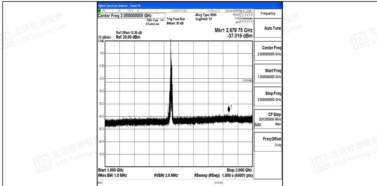
Band2_20MHz_QPSK_19100_1RB#0_1000~3000_1000~3000
