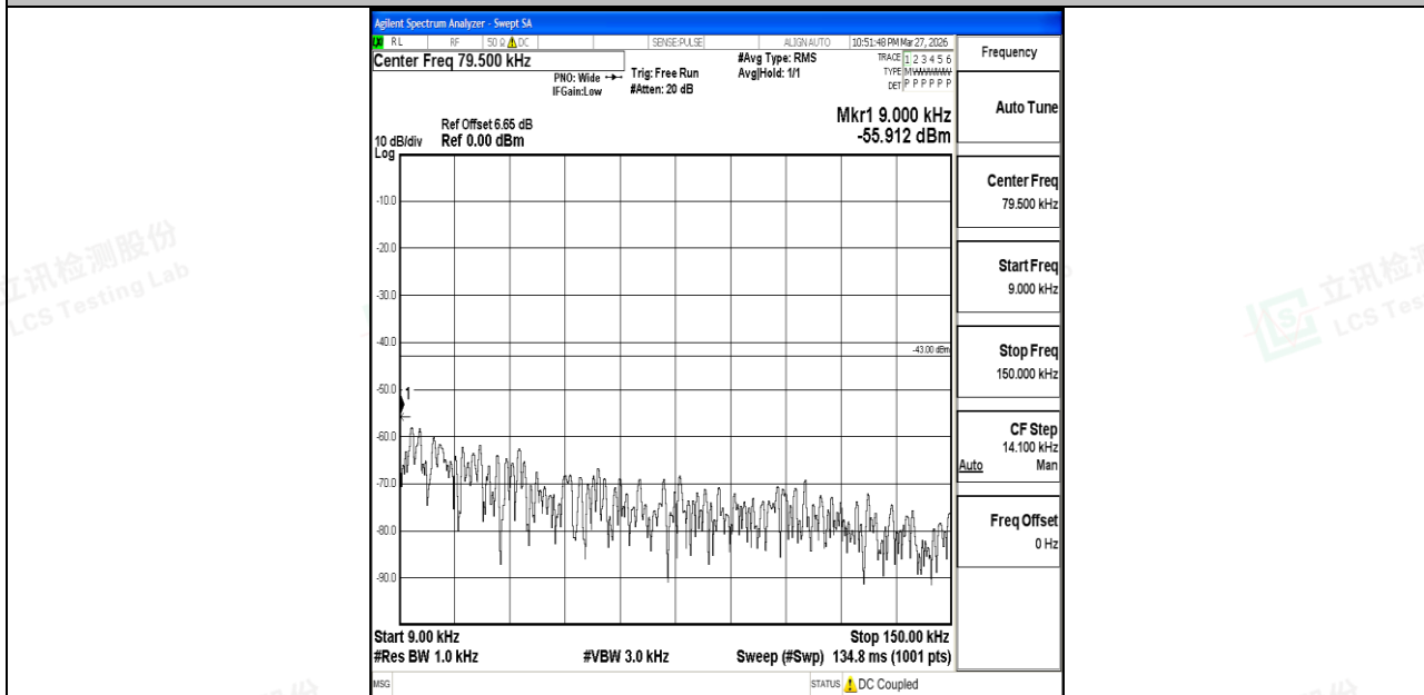
Band4_10MHz_QPSK_20350_1RB#0_0.009~0.15_0.009~0.15
