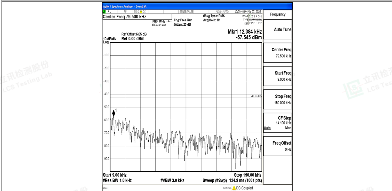
Band4_5MHz_QPSK_20375_1RB#0_0.009~0.15_0.009~0.15
