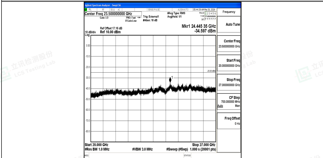
Band38_5MHz_16QAM_38225_1RB#0_20000~27000_20000~27000
