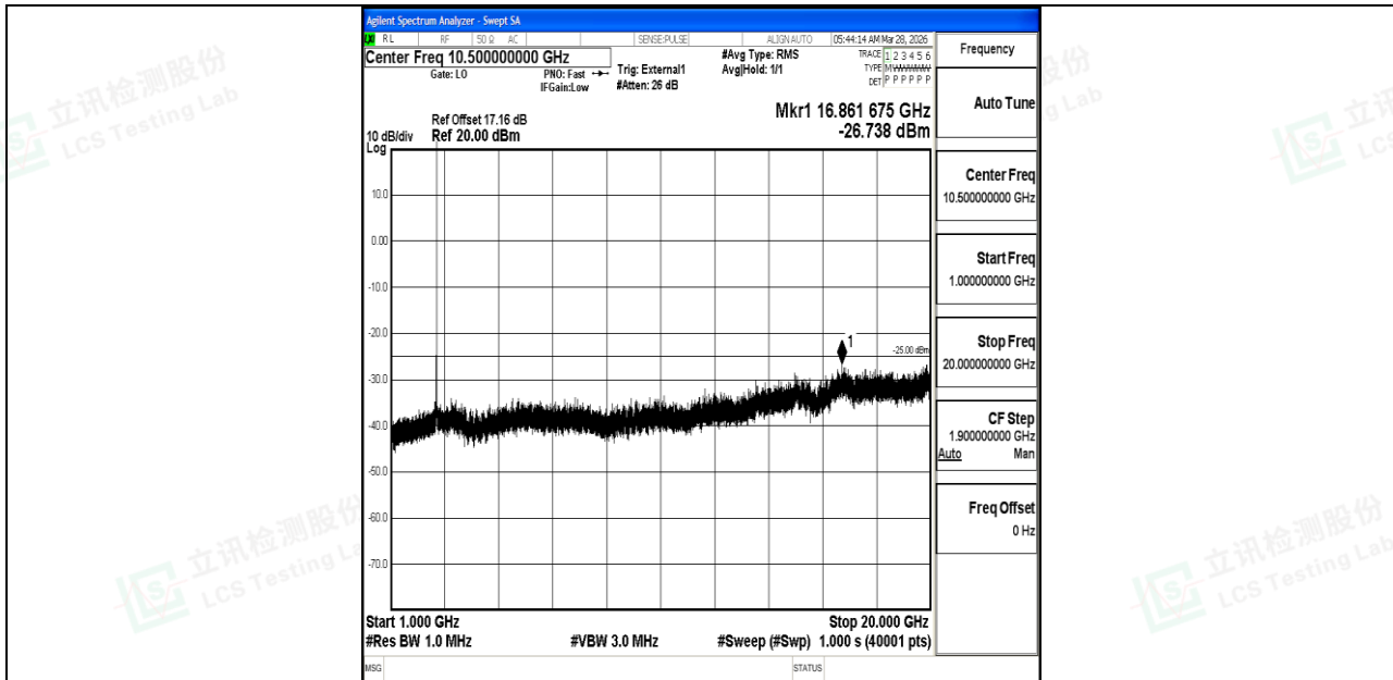
Band38_5MHz_16QAM_38225_1RB#0_1000~20000_1000~20000
