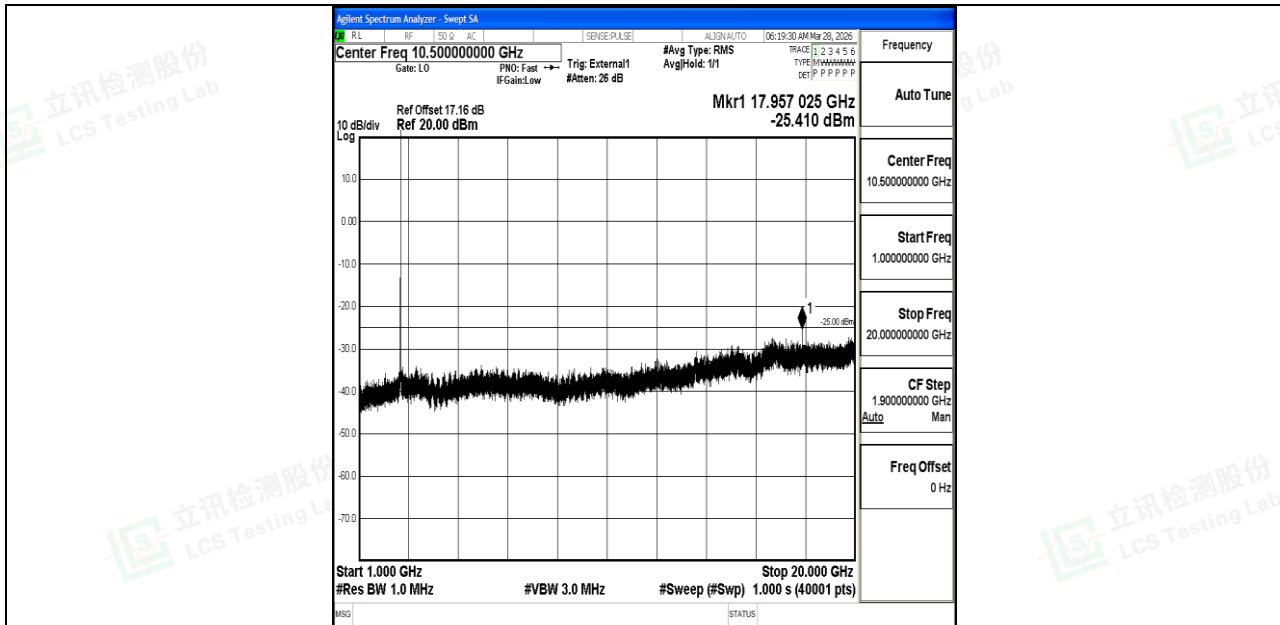
Band38_10MHz_16QAM_38000_1RB#0_1000~20000_1000~20000
