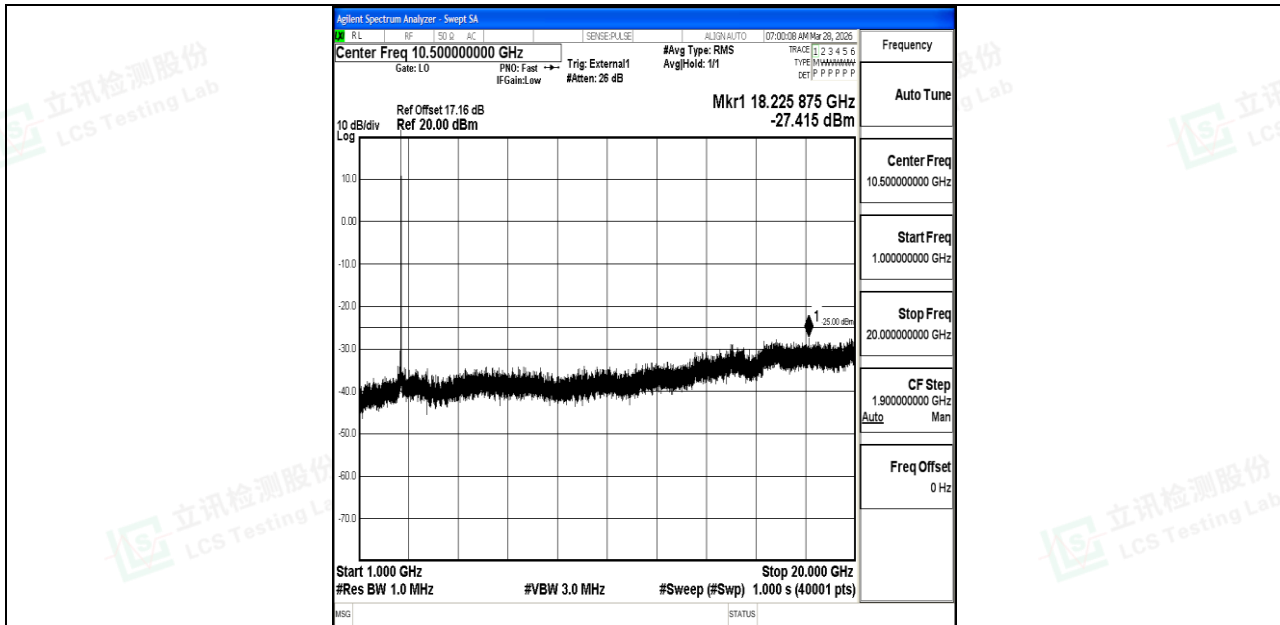
Band38_15MHz_16QAM_38175_1RB#0_1000~20000_1000~20000
