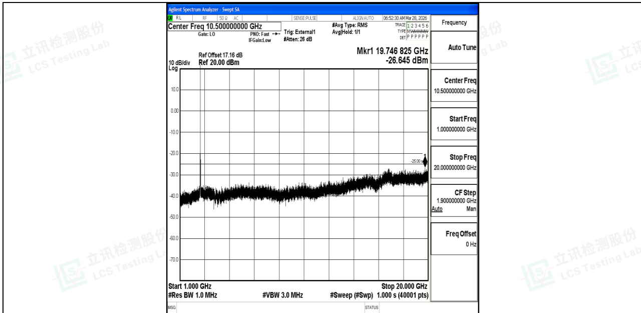
Band38_15MHz_16QAM_37825_1RB#0_1000~20000_1000~20000
