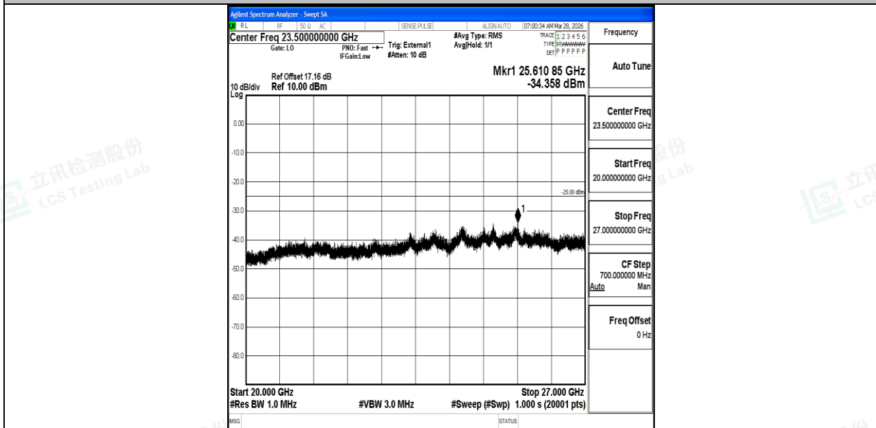
Band38_15MHz_16QAM_38175_1RB#0_20000~27000_20000~27000
