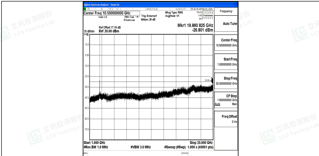
Band38_5MHz_16QAM_37775_1RB#0_1000~20000_1000~20000
