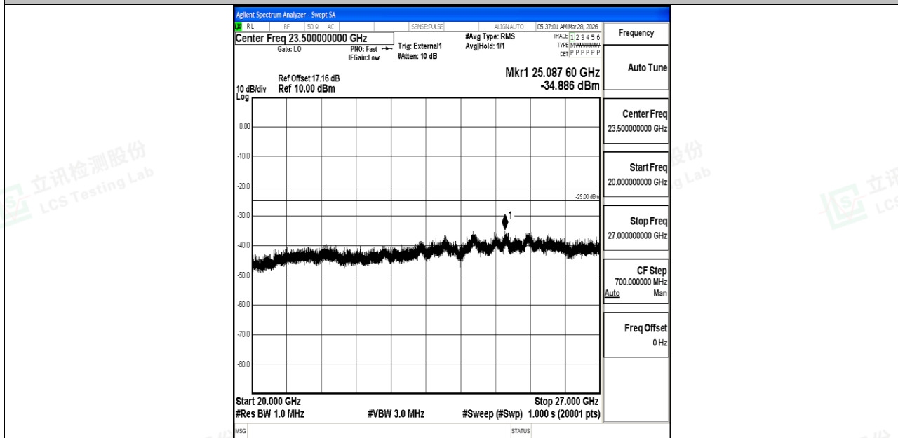
Band38_5MHz_16QAM_37775_1RB#0_20000~27000_20000~27000
