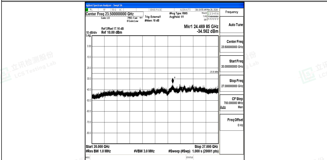
Band38_10MHz_16QAM_38000_1RB#0_20000~27000_20000~27000
