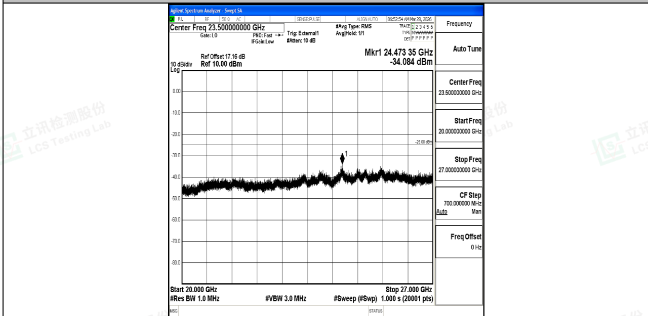
Band38_15MHz_16QAM_37825_1RB#0_20000~27000_20000~27000
