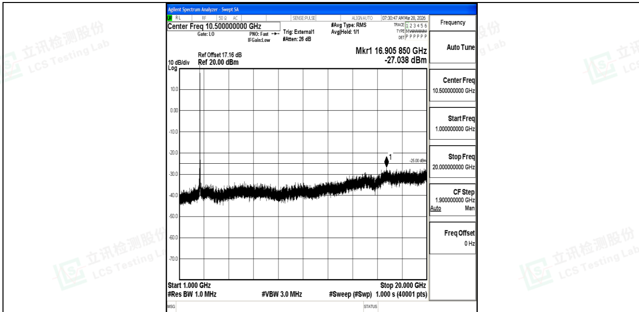
Band38_20MHz_16QAM_38000_1RB#0_1000~20000_1000~20000
