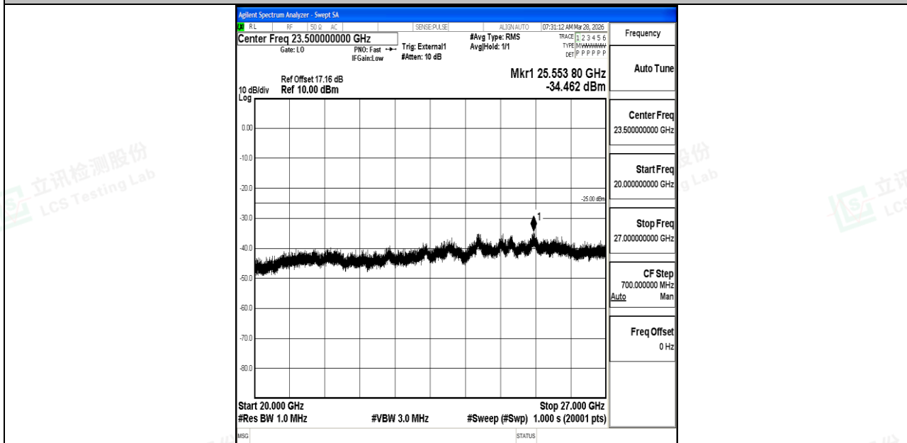
Band38_20MHz_16QAM_38000_1RB#0_20000~27000_20000~27000
