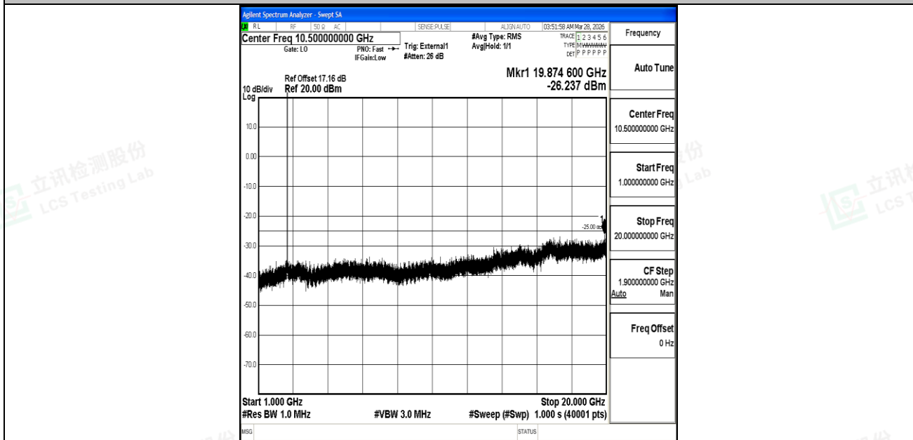
Band41_10MHz_QPSK_40620_1RB#0_1000~20000_1000~20000
