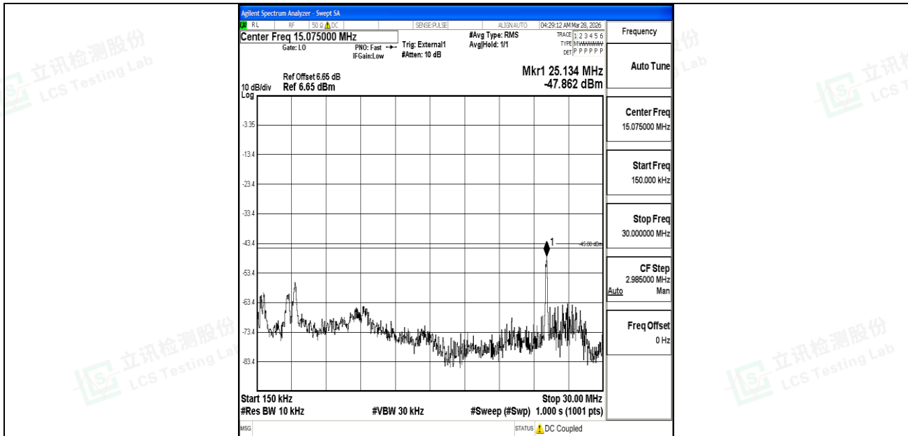
Band41_15MHz_16QAM_40620_1RB#0_0.15~30_0.15~30
