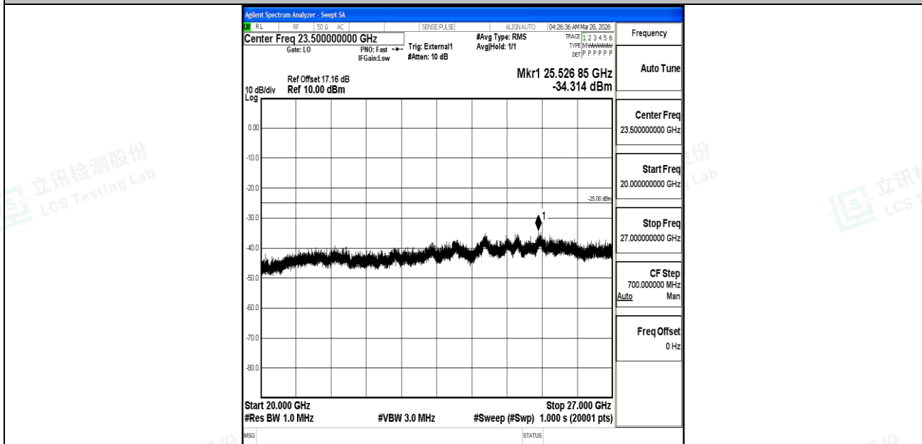
Band41_15MHz_16QAM_39725_1RB#0_20000~27000_20000~27000
