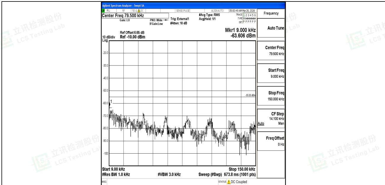
Band41_20MHz_QPSK_40620_1RB#0_0.009~0.15_0.009~0.15
