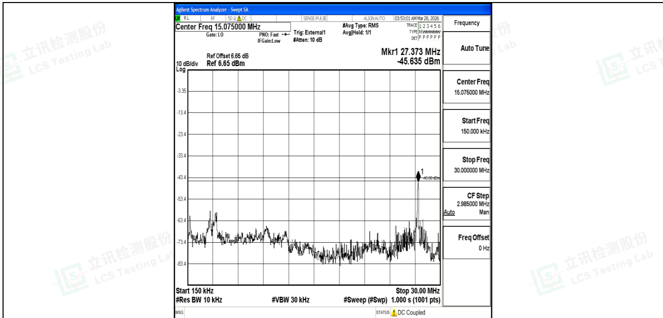
Band41_10MHz_16QAM_40620_1RB#0_0.15~30_0.15~30
