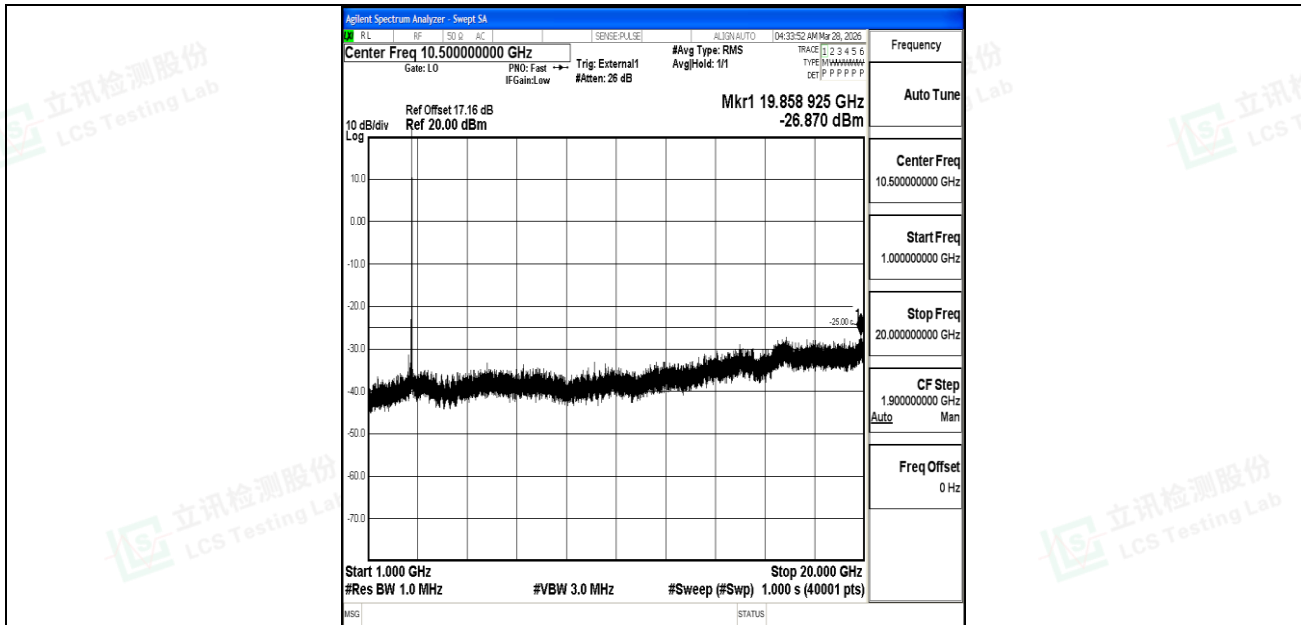
Band41_15MHz_16QAM_41515_1RB#0_1000~20000_1000~20000
