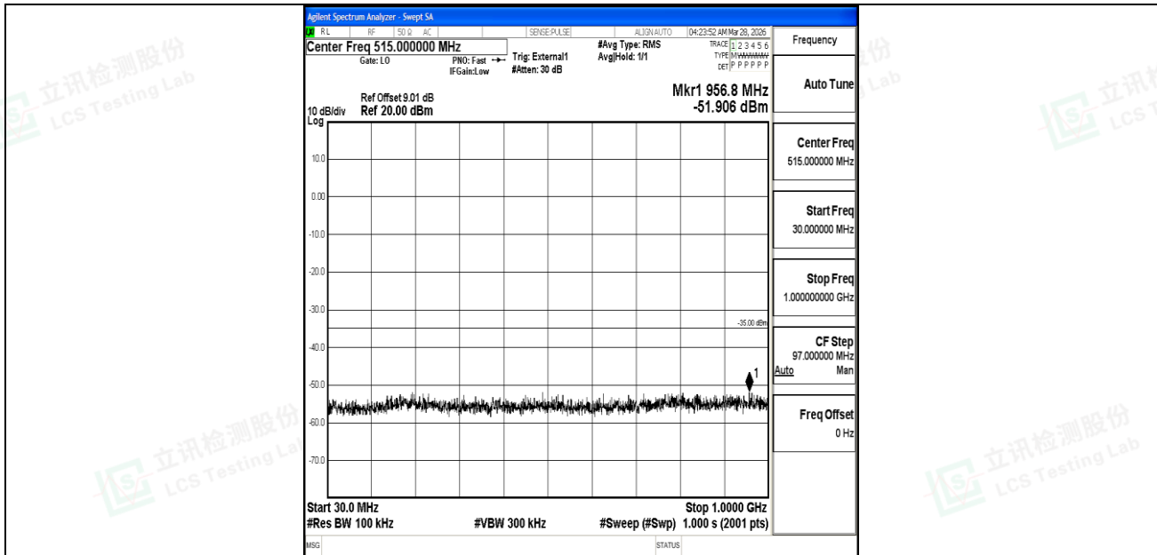
Band41_15MHz_QPSK_39725_1RB#0_30~1000_30~1000
