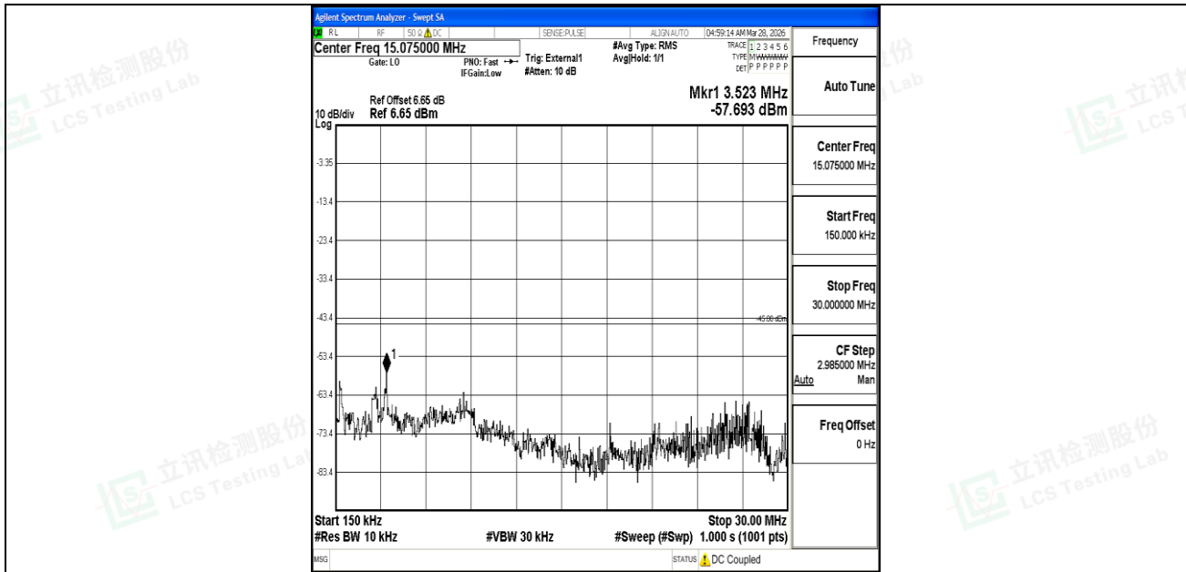
Band41_20MHz_16QAM_39750_1RB#0_0.15~30_0.15~30
