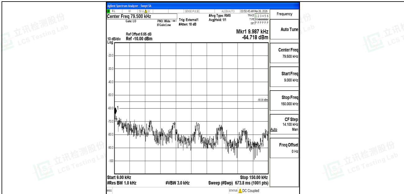
Band41_10MHz_QPSK_40620_1RB#0_0.009~0.15_0.009~0.15
