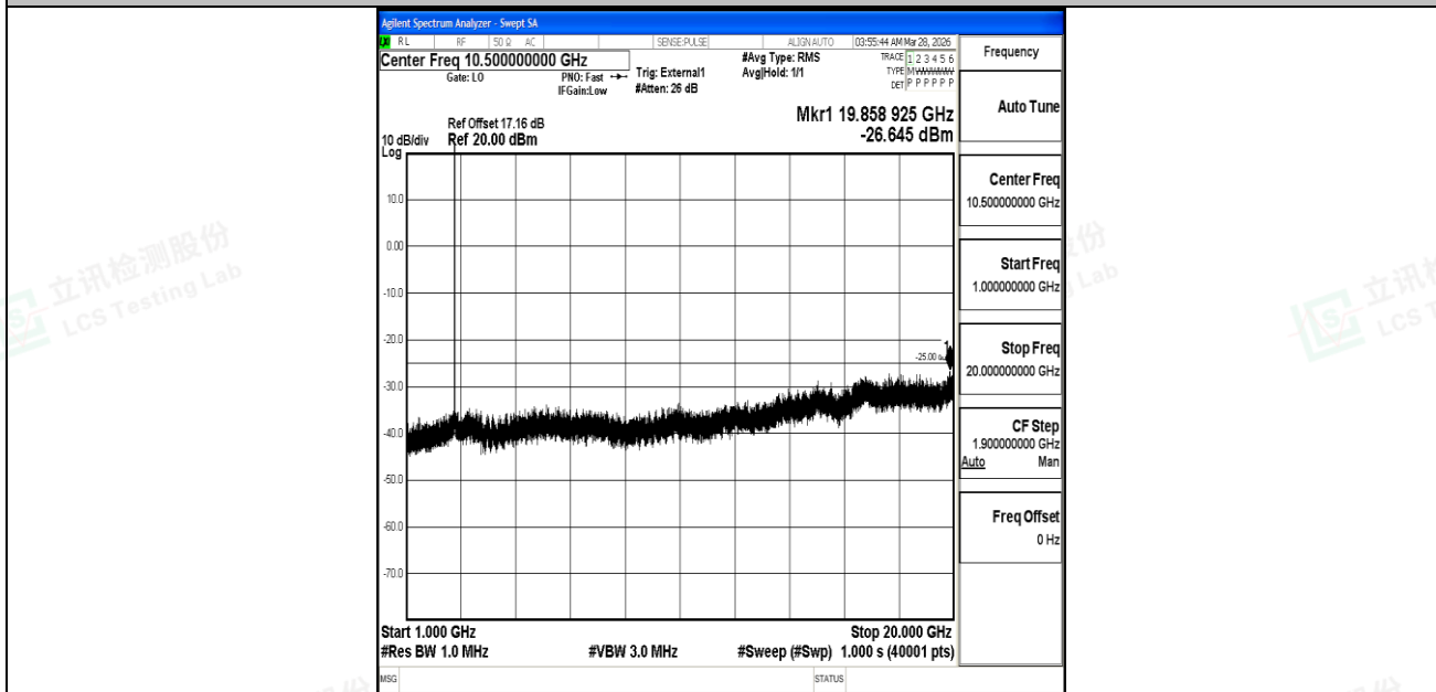
Band41_10MHz_QPSK_41540_1RB#0_1000~20000_1000~20000
