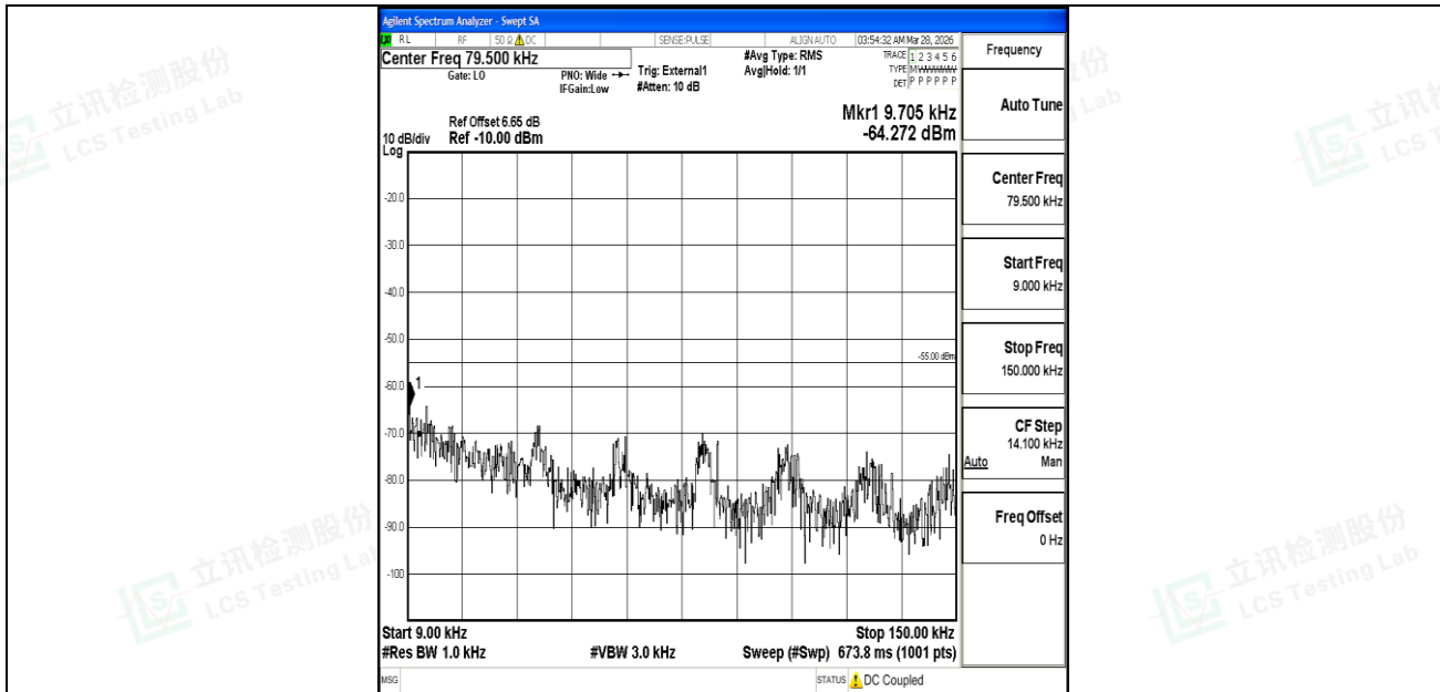
Band41_10MHz_QPSK_41540_1RB#0_0.009~0.15_0.009~0.15
