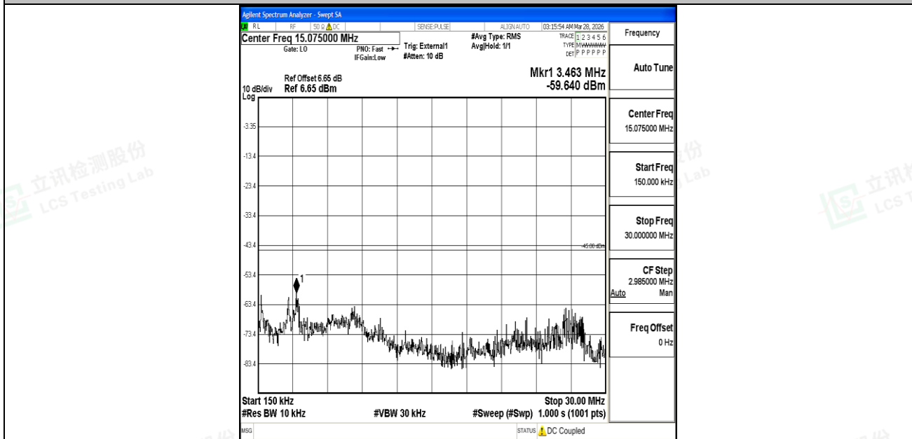
Band41_5MHz_QPSK_41565_1RB#0_0.15~30_0.15~30
