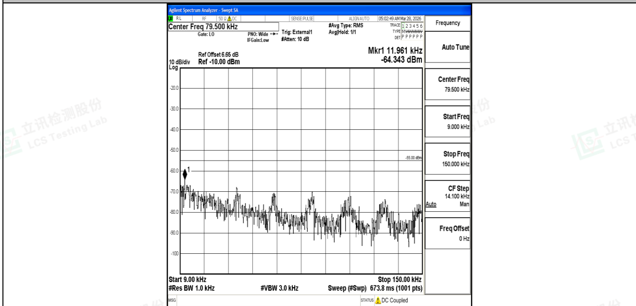
Band41_20MHz_16QAM_40620_1RB#0_0.009~0.15_0.009~0.15
