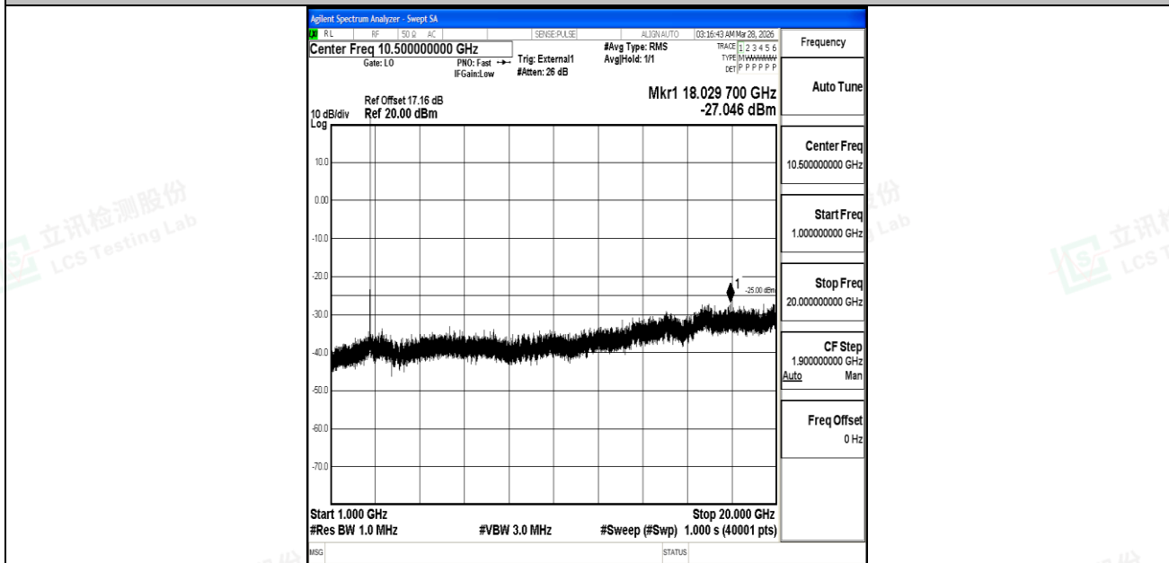
Band41_5MHz_QPSK_41565_1RB#0_1000~20000_1000~20000
