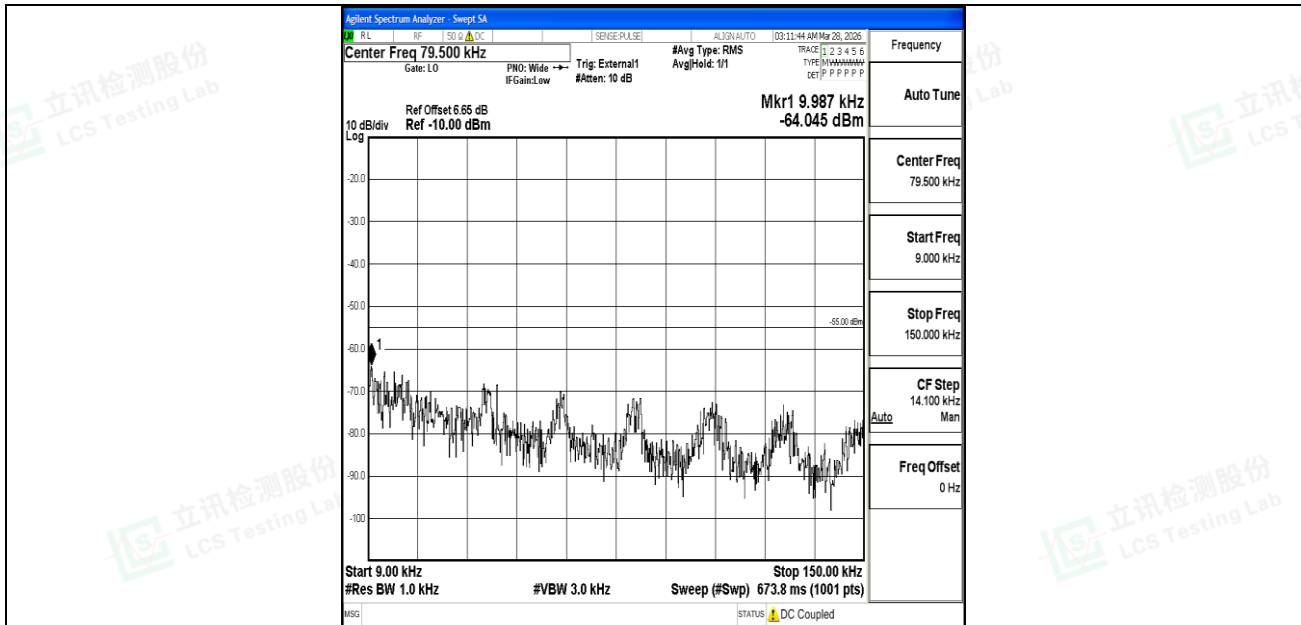
Band41_5MHz_QPSK_40620_1RB#0_0.009~0.15_0.009~0.15
