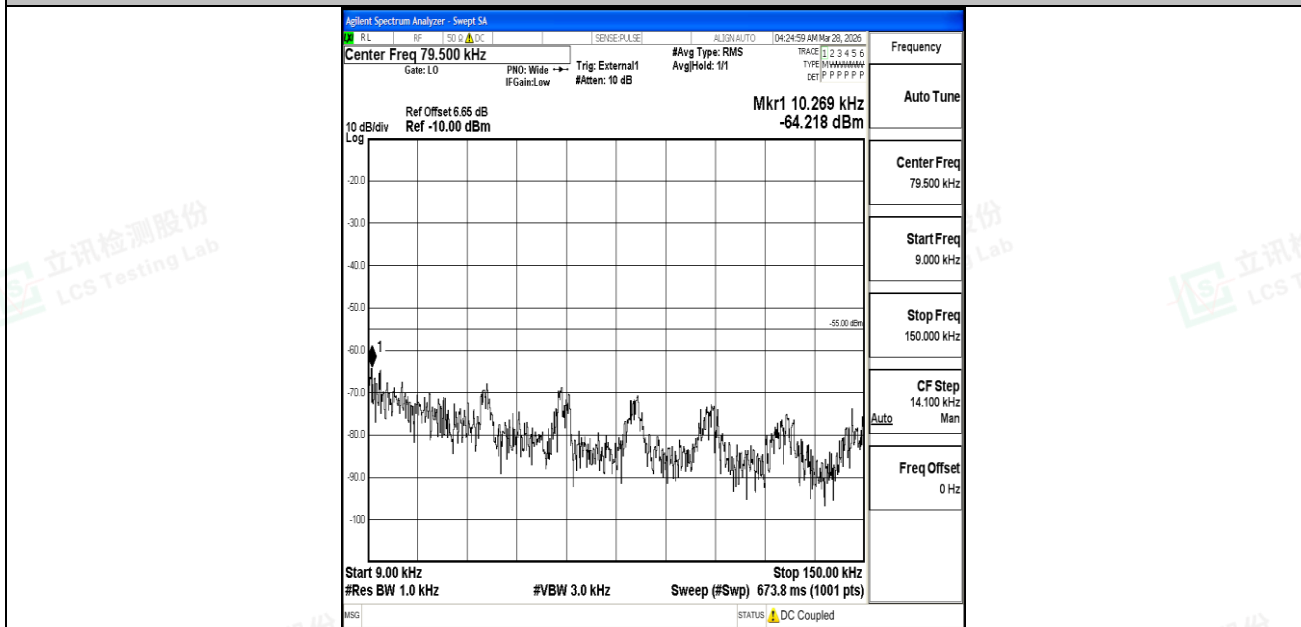
Band41_15MHz_16QAM_39725_1RB#0_0.009~0.15_0.009~0.15
