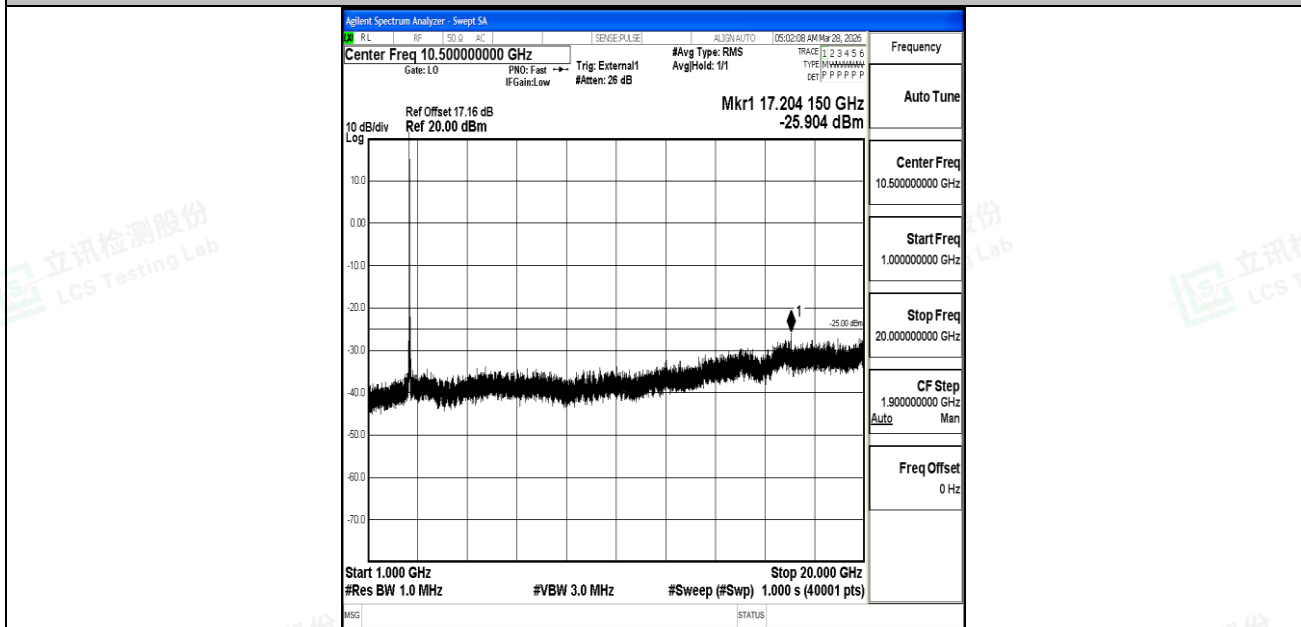
Band41_20MHz_QPSK_40620_1RB#0_1000~20000_1000~20000
