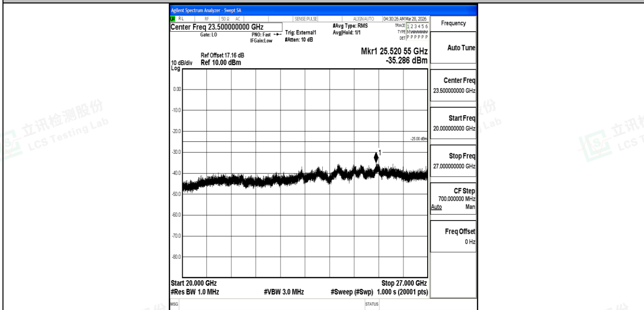
Band41_15MHz_16QAM_40620_1RB#0_20000~27000_20000~27000
