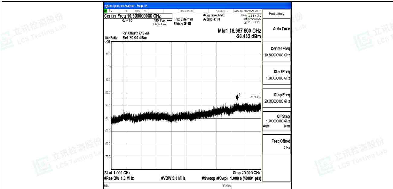
Band41_10MHz_16QAM_39700_1RB#0_1000~20000_1000~20000
