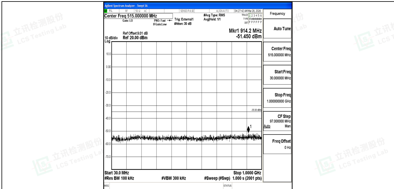
Band41_15MHz_QPSK_40620_1RB#0_30~1000_30~1000
