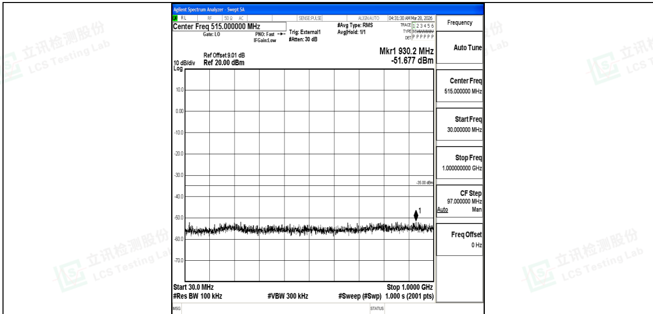
Band41_15MHz_QPSK_41515_1RB#0_30~1000_30~1000
