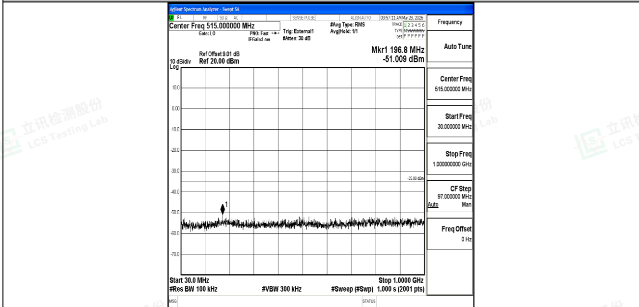
Band41_10MHz_16QAM_41540_1RB#0_30~1000_30~1000
