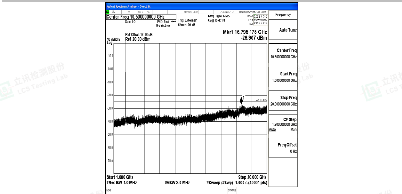
Band41_10MHz_QPSK_39700_1RB#0_1000~20000_1000~20000
