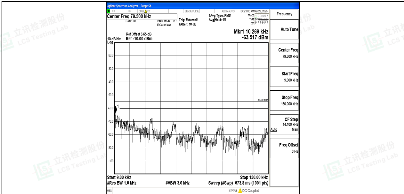
Band41_15MHz_QPSK_39725_1RB#0_0.009~0.15_0.009~0.15
