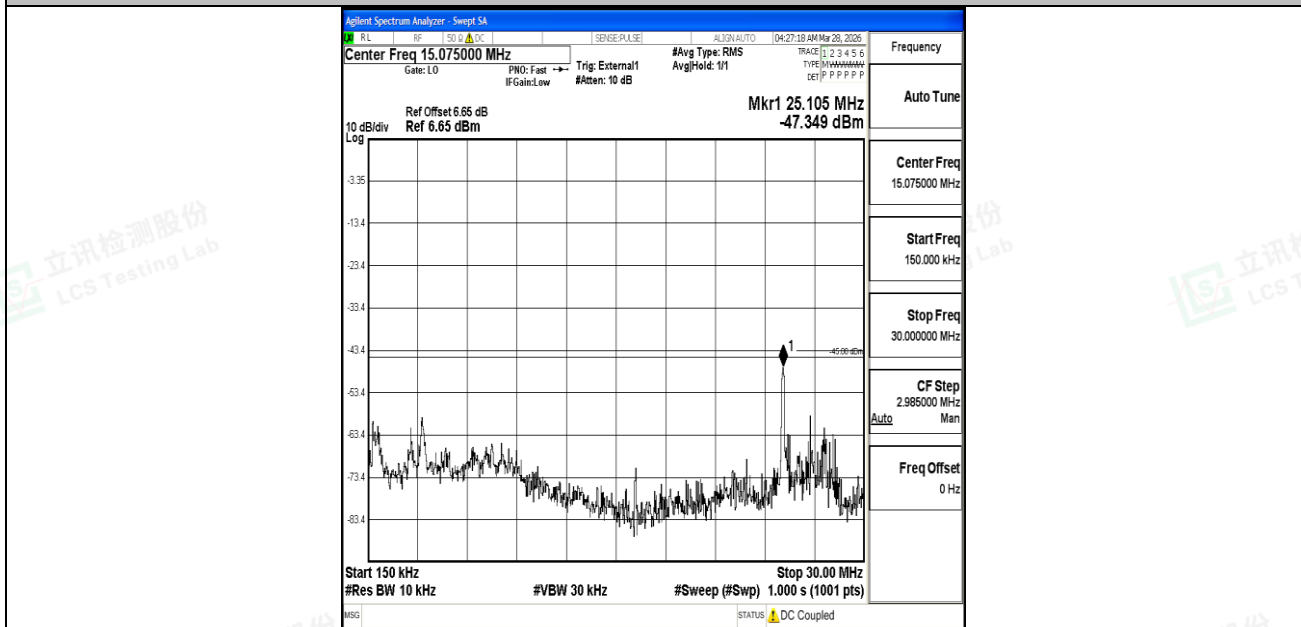
Band41_15MHz_QPSK_40620_1RB#0_0.15~30_0.15~30
