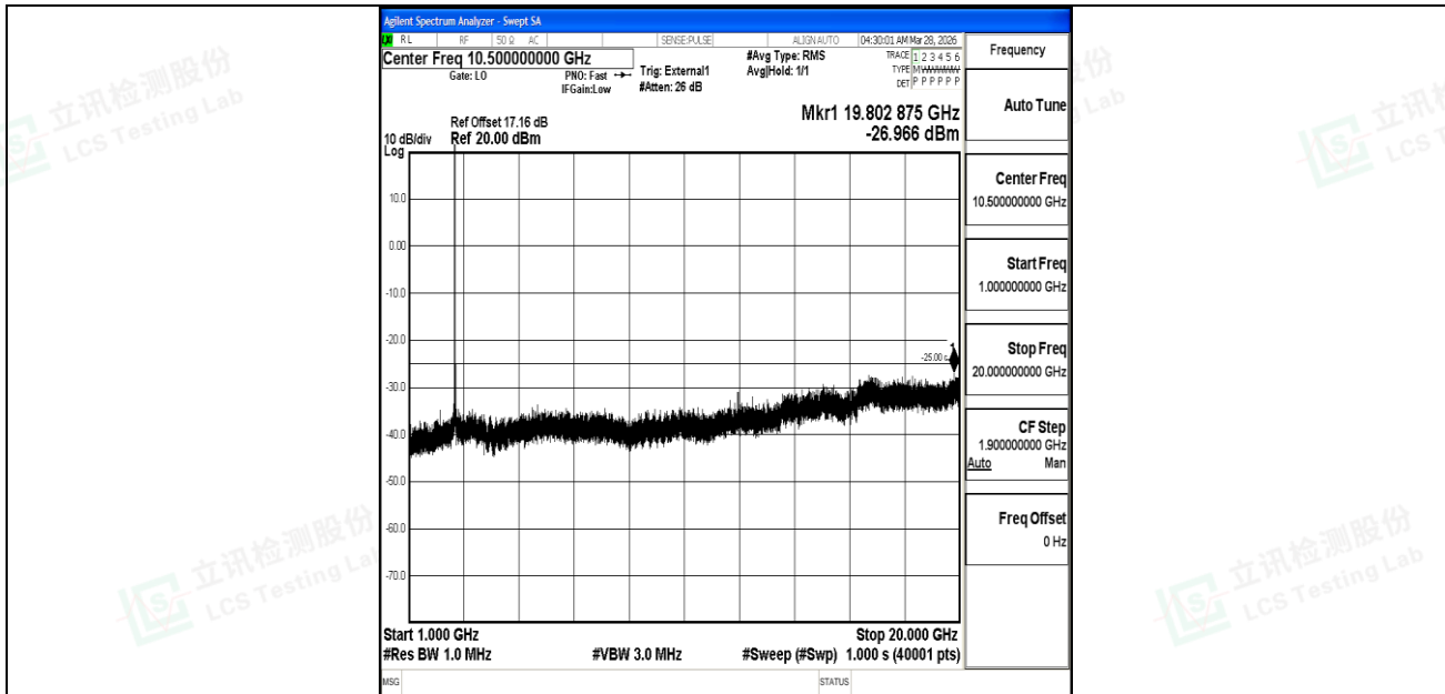
Band41_15MHz_16QAM_40620_1RB#0_1000~20000_1000~20000
