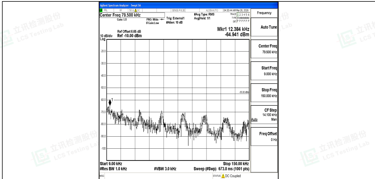
Band41_15MHz_QPSK_41515_1RB#0_0.009~0.15_0.009~0.15
