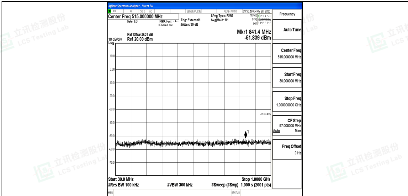
Band41_10MHz_QPSK_41540_1RB#0_30~1000_30~1000
