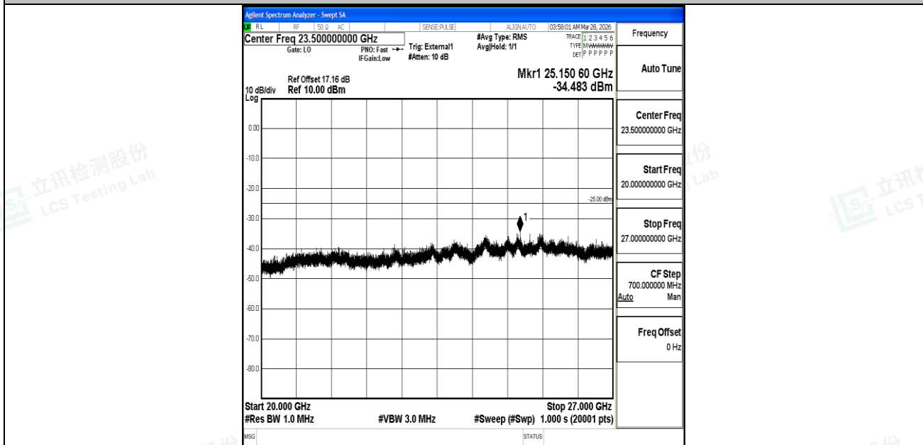
Band41_10MHz_16QAM_41540_1RB#0_20000~27000_20000~27000
