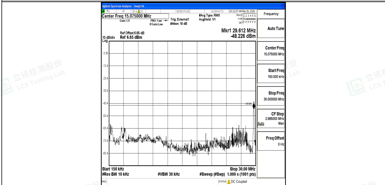
Band41_5MHz_QPSK_40620_1RB#0_0.15~30_0.15~30
