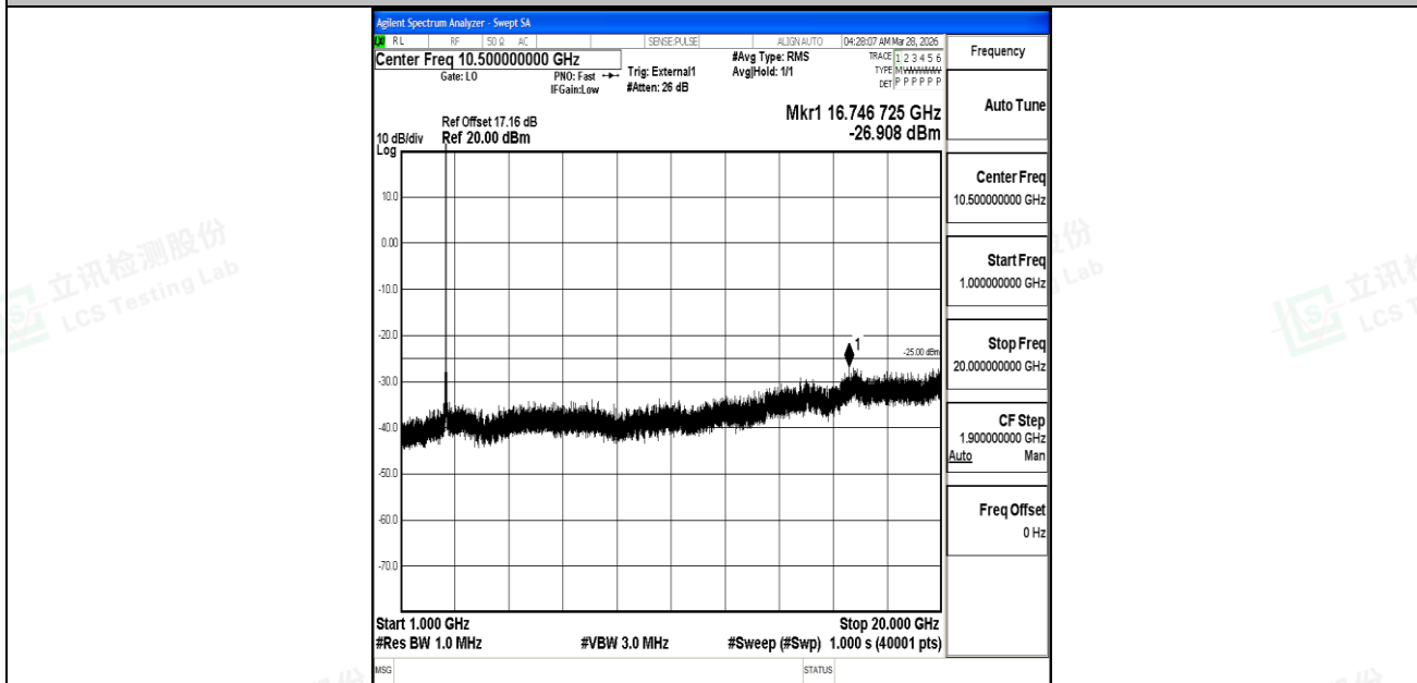
Band41_15MHz_QPSK_40620_1RB#0_1000~20000_1000~20000
