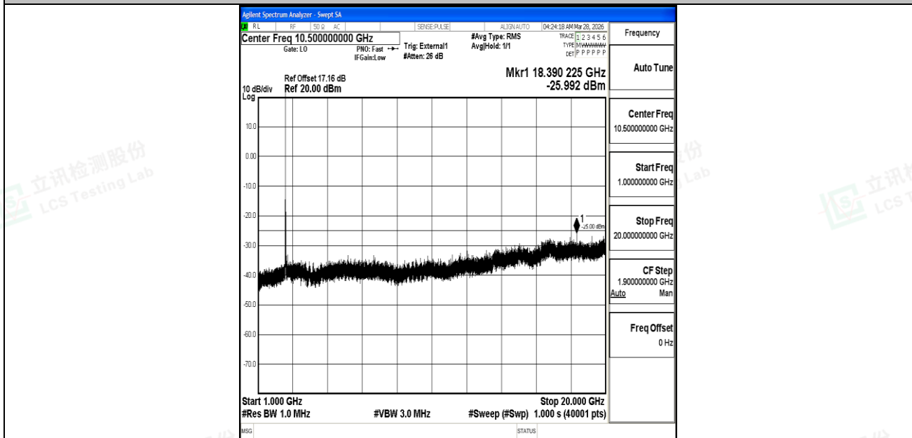
Band41_15MHz_QPSK_39725_1RB#0_1000~20000_1000~20000
