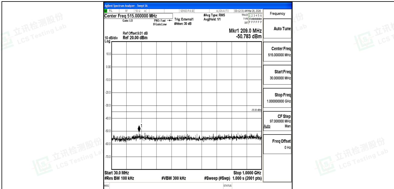
Band41_5MHz_QPSK_40620_1RB#0_30~1000_30~1000
