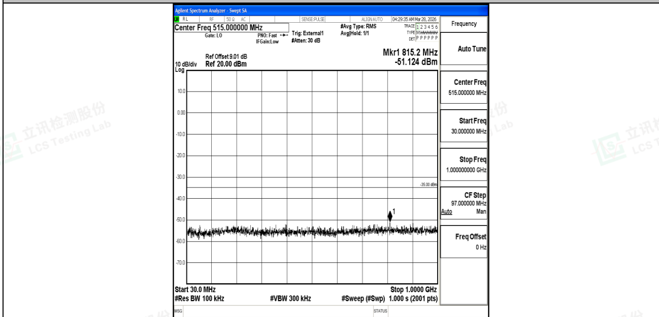
Band41_15MHz_16QAM_40620_1RB#0_30~1000_30~1000
