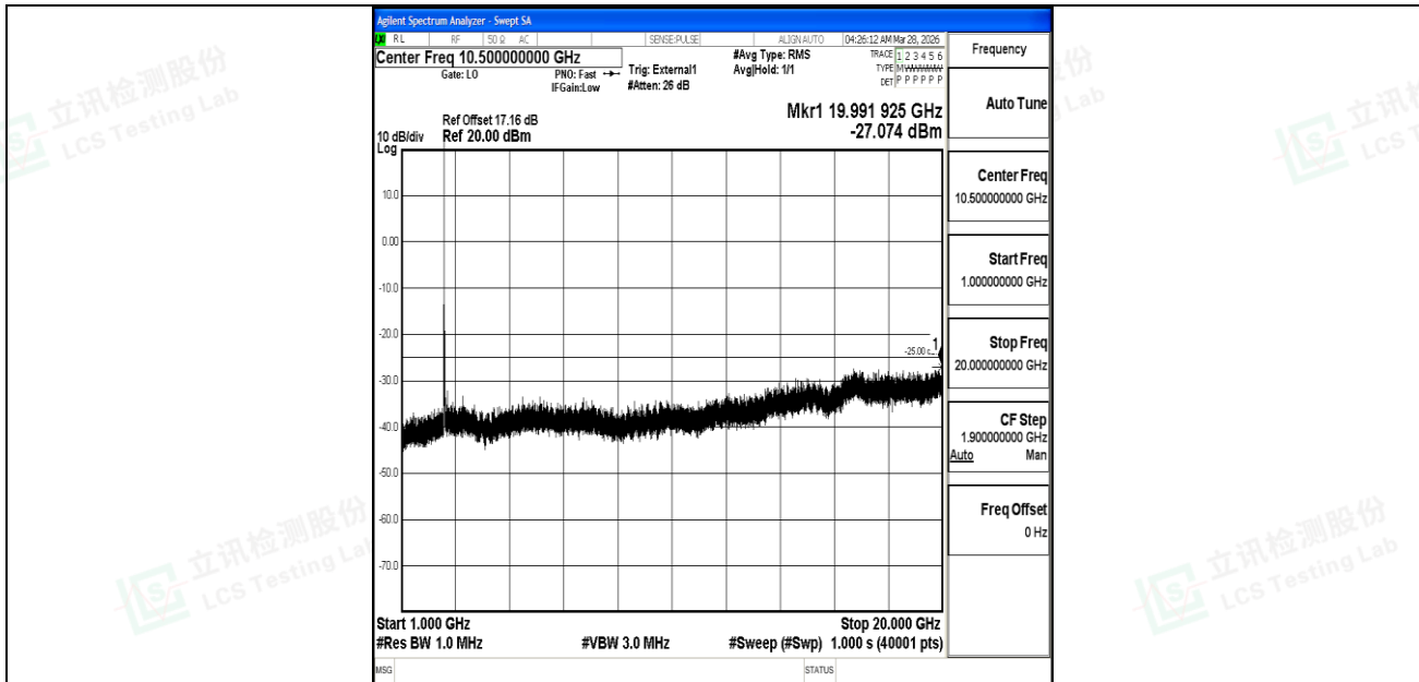
Band41_15MHz_16QAM_39725_1RB#0_1000~20000_1000~20000
