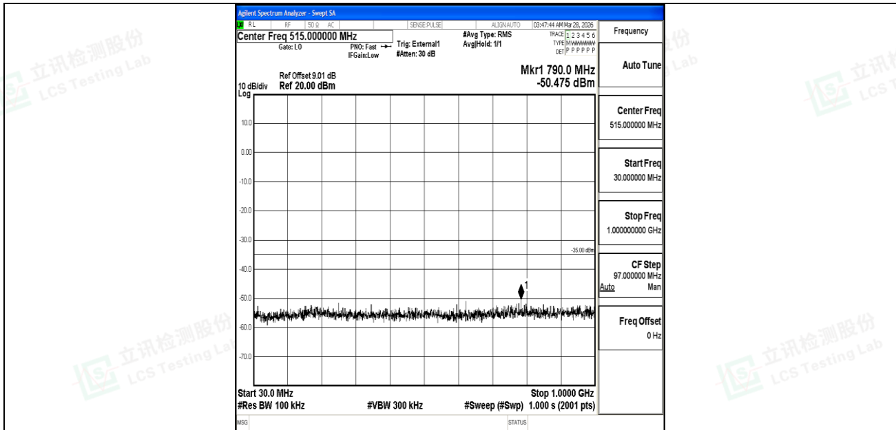
Band41_10MHz_QPSK_39700_1RB#0_30~1000_30~1000
