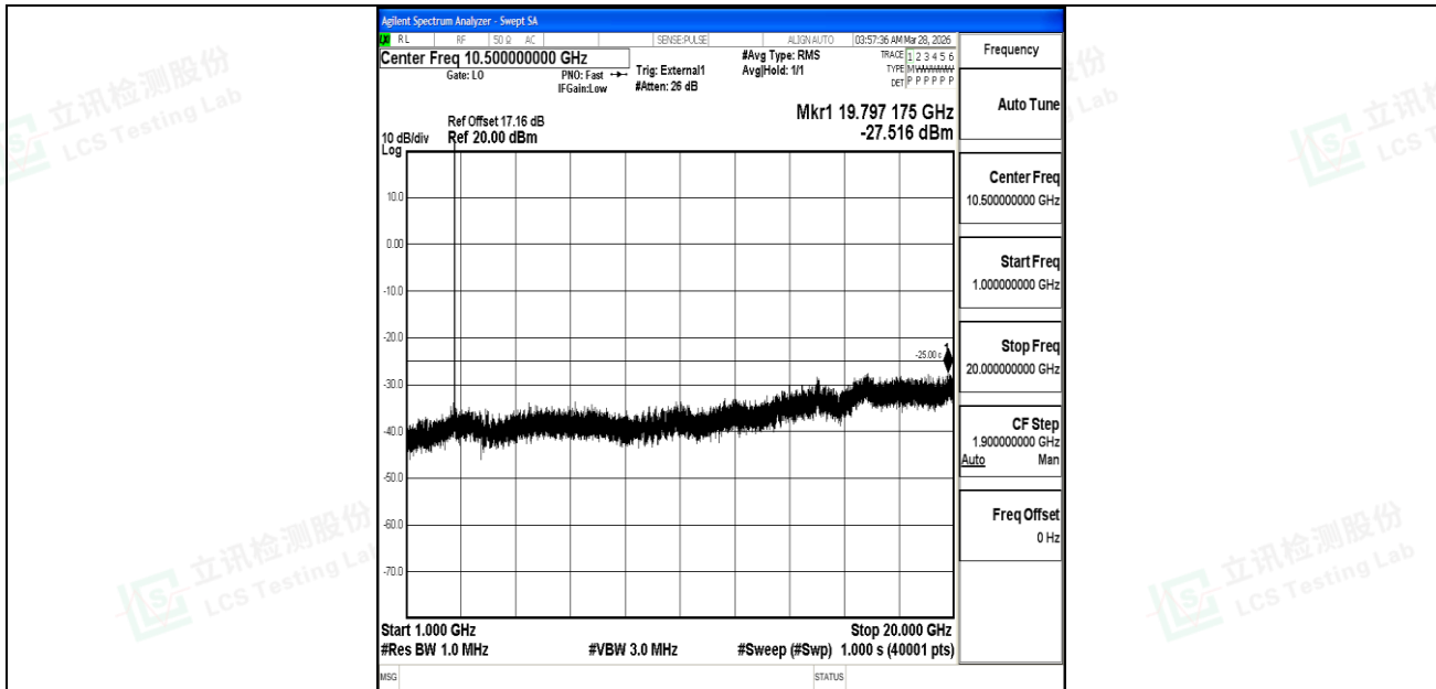
Band41_10MHz_16QAM_41540_1RB#0_1000~20000_1000~20000
