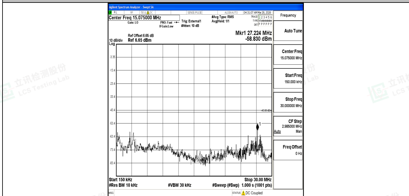
Band41_15MHz_QPSK_41515_1RB#0_0.15~30_0.15~30
