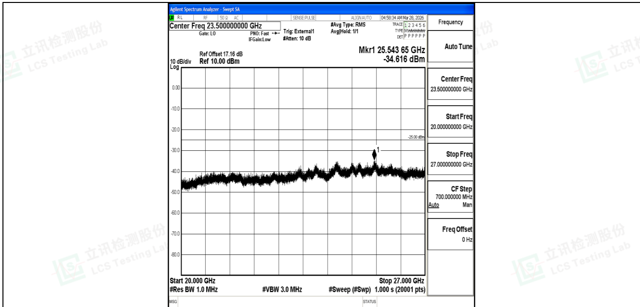
Band41_20MHz_QPSK_39750_1RB#0_20000~27000_20000~27000
