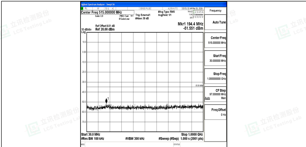
Band41_10MHz_QPSK_40620_1RB#0_30~1000_30~1000
