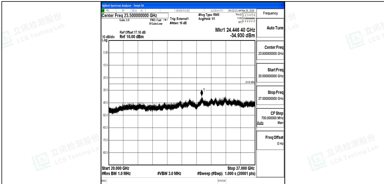
Band41_15MHz_QPSK_41515_1RB#0_20000~27000_20000~27000
