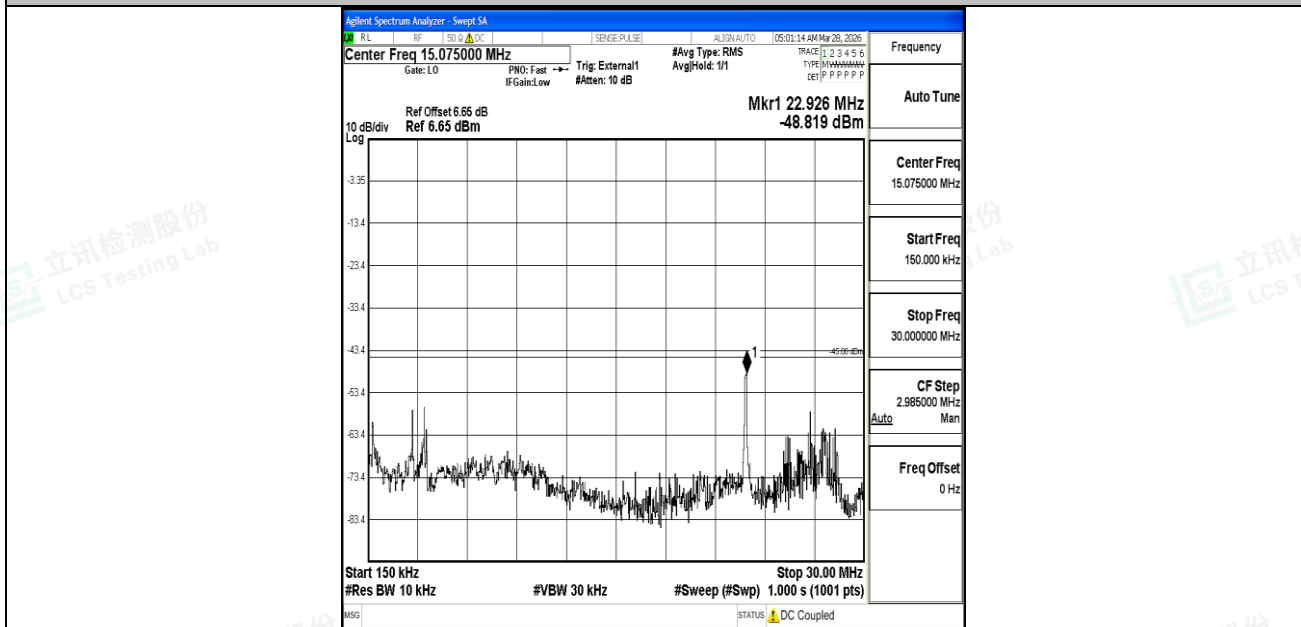
Band41_20MHz_QPSK_40620_1RB#0_0.15~30_0.15~30
