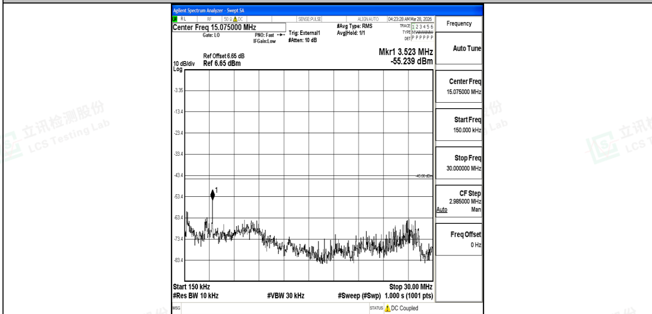
Band41_15MHz_QPSK_39725_1RB#0_0.15~30_0.15~30
