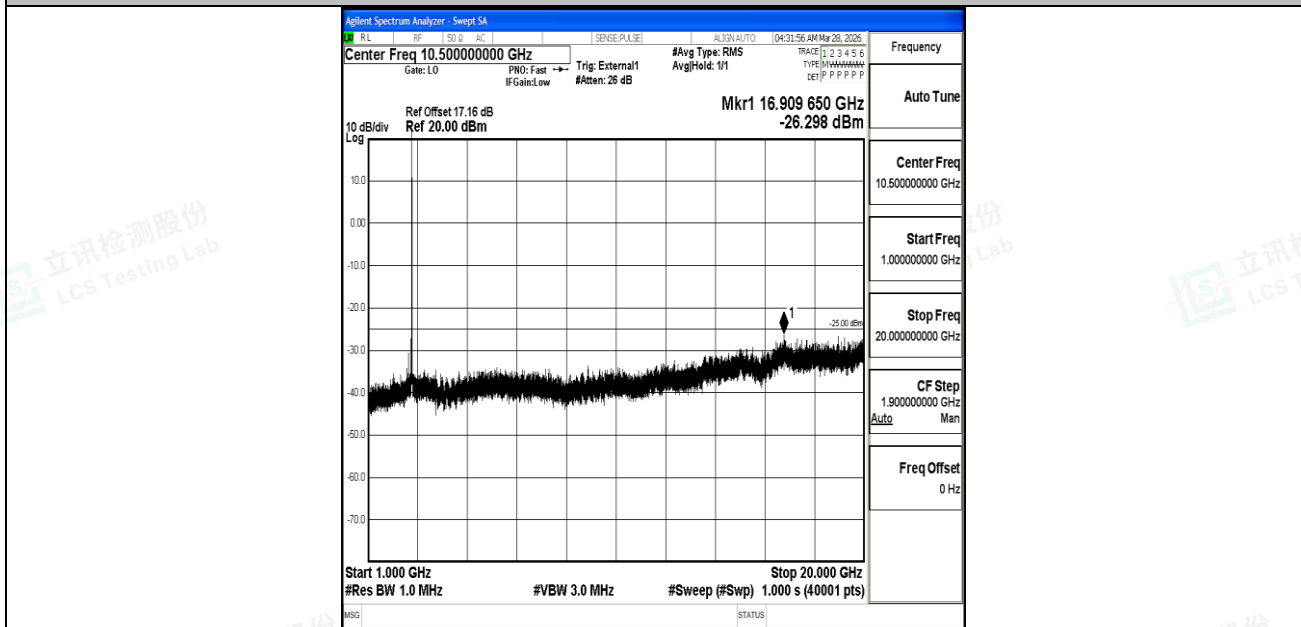
Band41_15MHz_QPSK_41515_1RB#0_1000~20000_1000~20000
