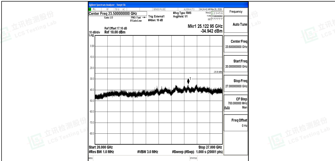
Band41_15MHz_QPSK_39725_1RB#0_20000~27000_20000~27000
