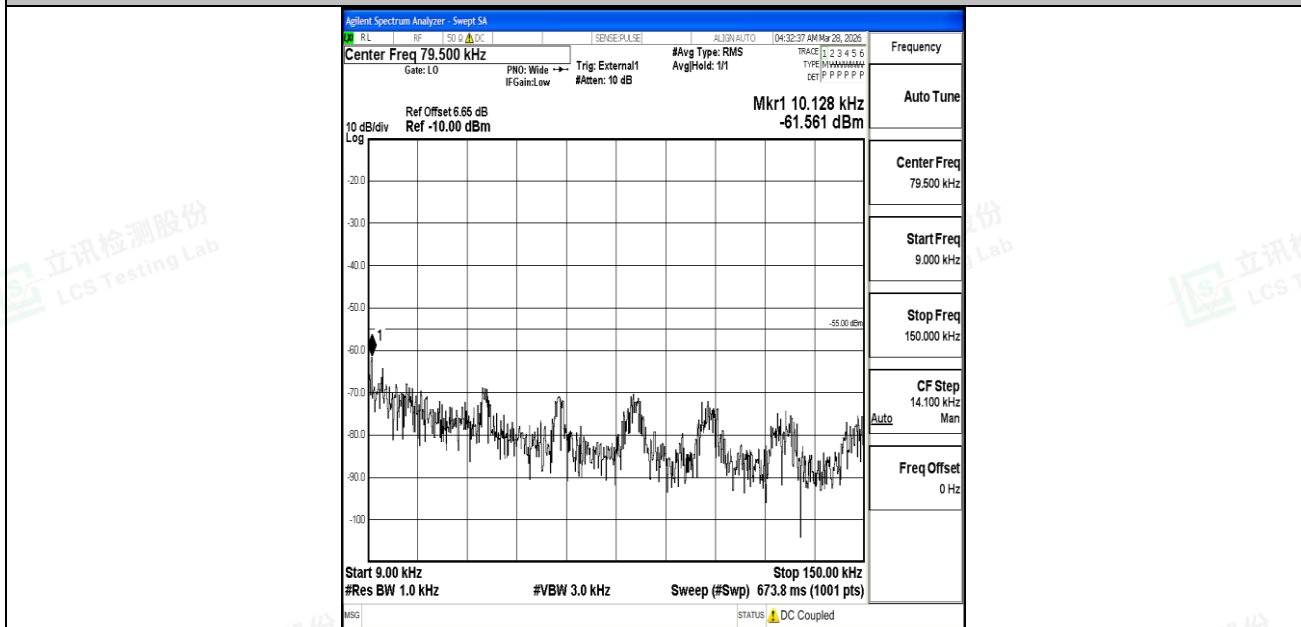
Band41_15MHz_16QAM_41515_1RB#0_0.009~0.15_0.009~0.15
