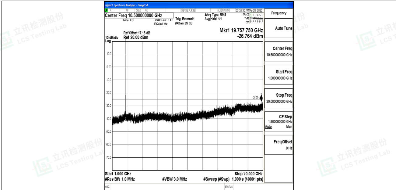
Band41_5MHz_16QAM_41565_1RB#0_1000~20000_1000~20000
