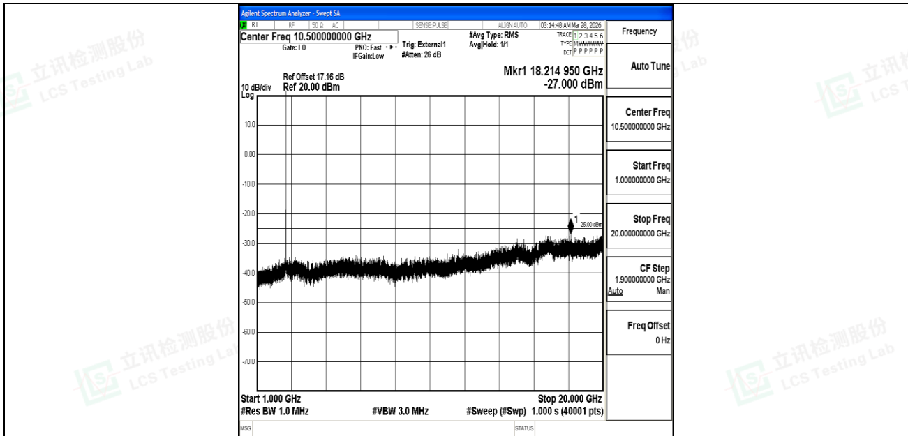
Band41_5MHz_16QAM_40620_1RB#0_1000~20000_1000~20000
