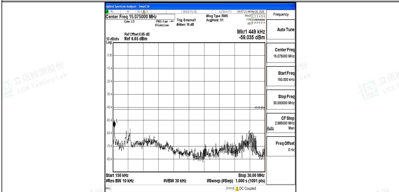
Band41_20MHz_QPSK_39750_1RB#0_0.15~30_0.15~30
