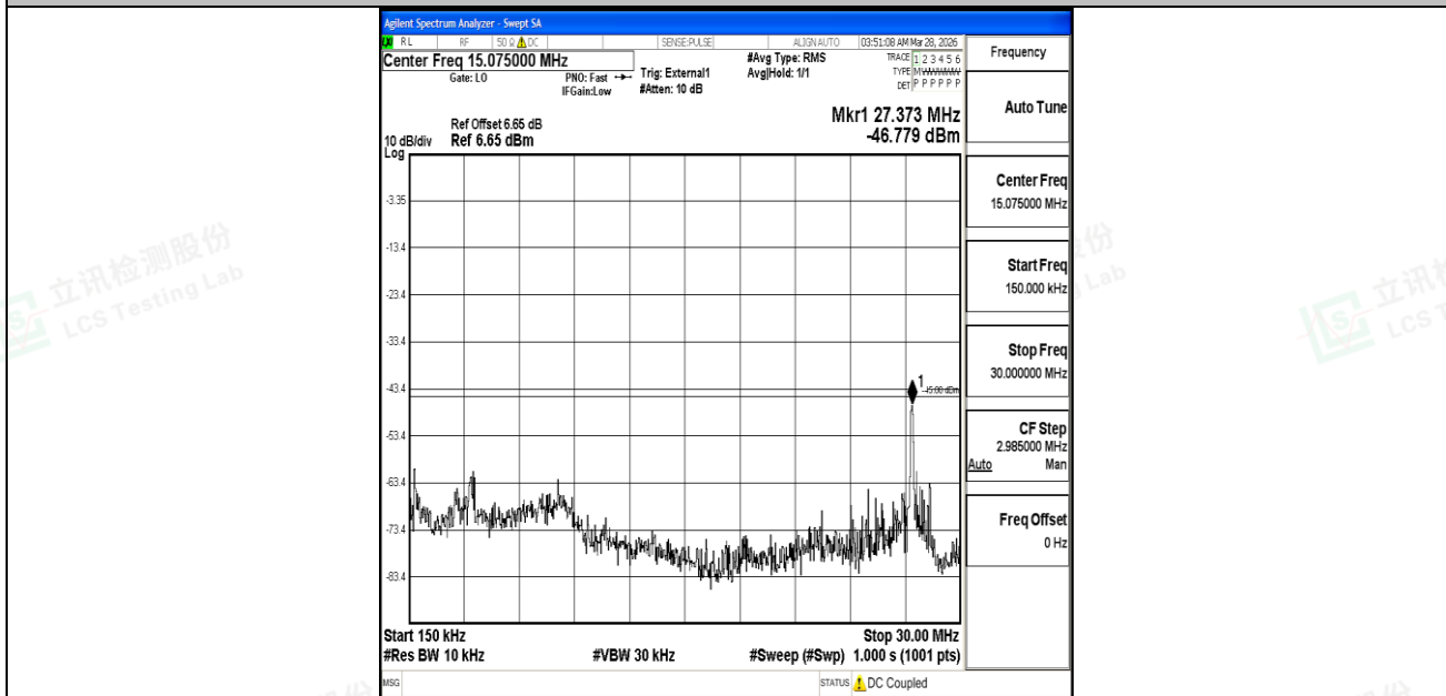
Band41_10MHz_QPSK_40620_1RB#0_0.15~30_0.15~30
