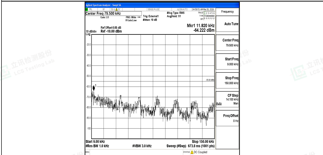
Band41_20MHz_16QAM_39750_1RB#0_0.009~0.15_0.009~0.15
