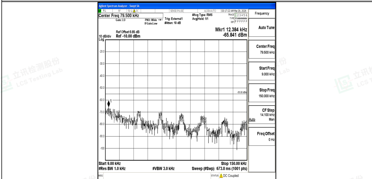
Band41_5MHz_16QAM_41565_1RB#0_0.009~0.15_0.009~0.15
