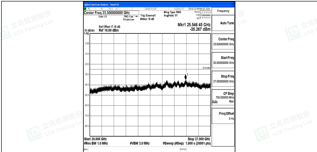
Band41_20MHz_QPSK_40620_1RB#0_20000~27000_20000~27000
