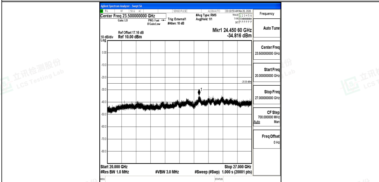
Band41_5MHz_16QAM_41565_1RB#0_20000~27000_20000~27000
