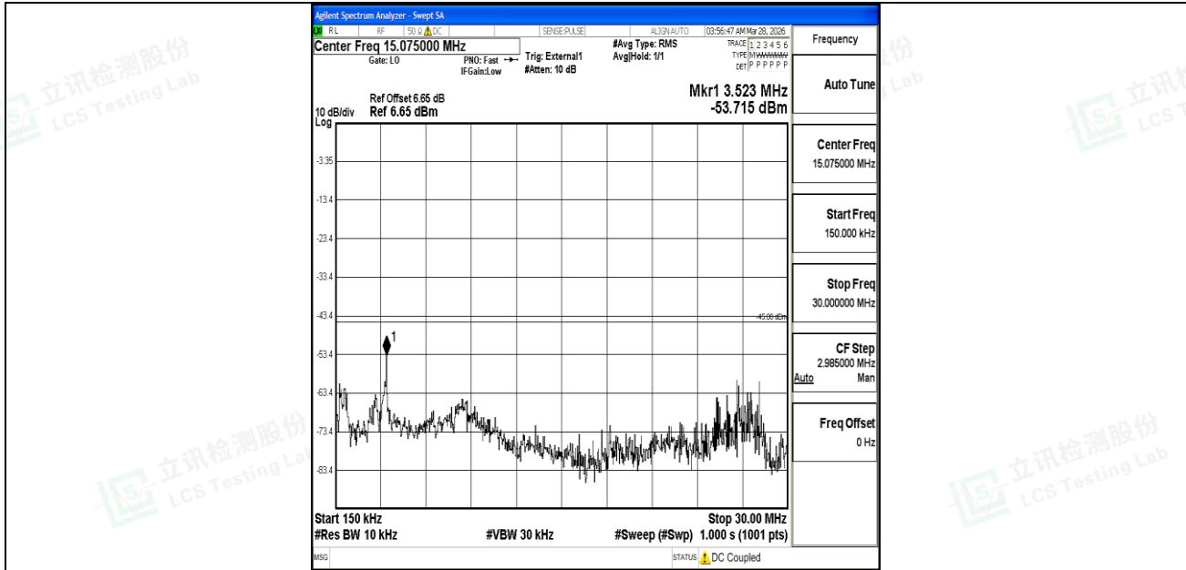
Band41_10MHz_16QAM_41540_1RB#0_0.15~30_0.15~30
