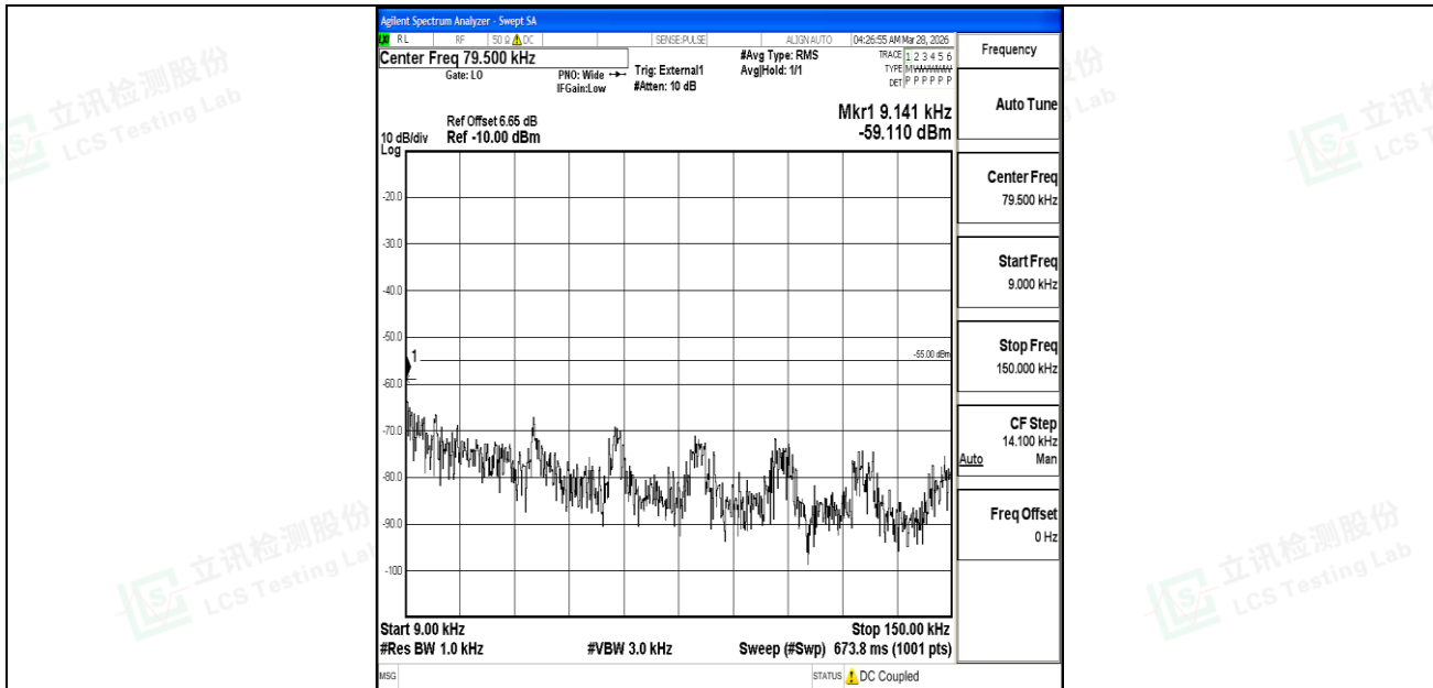
Band41_15MHz_QPSK_40620_1RB#0_0.009~0.15_0.009~0.15
