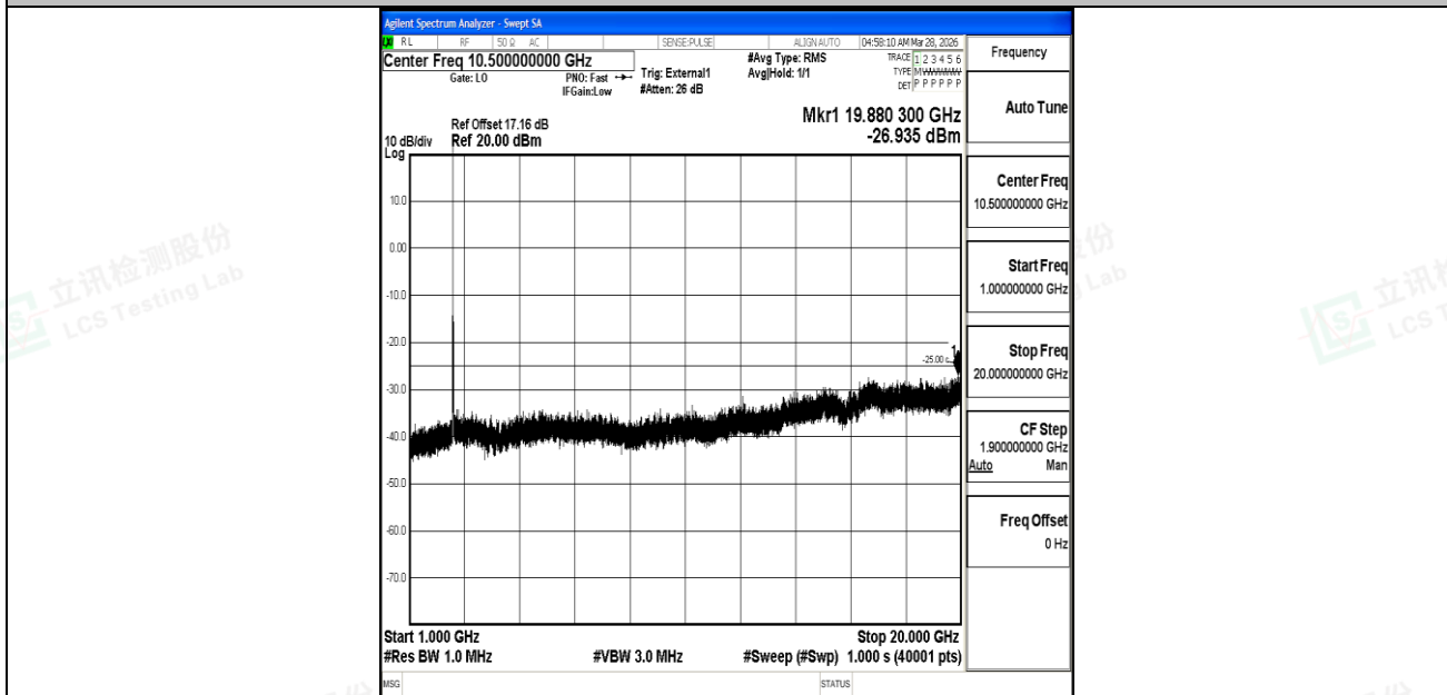
Band41_20MHz_QPSK_39750_1RB#0_1000~20000_1000~20000
