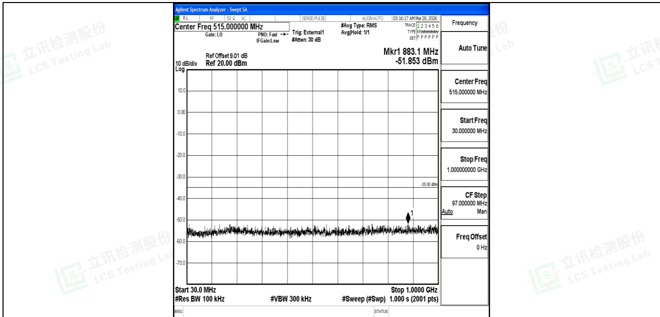
Band41_5MHz_QPSK_41565_1RB#0_30~1000_30~1000
