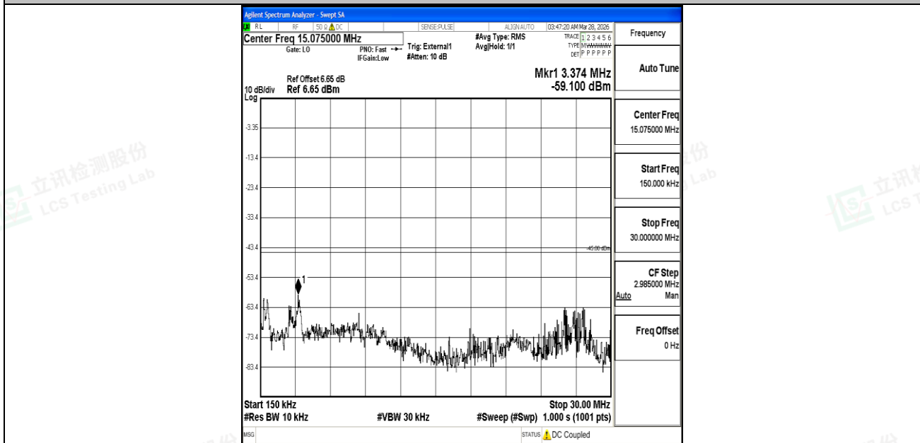
Band41_10MHz_QPSK_39700_1RB#0_0.15~30_0.15~30
