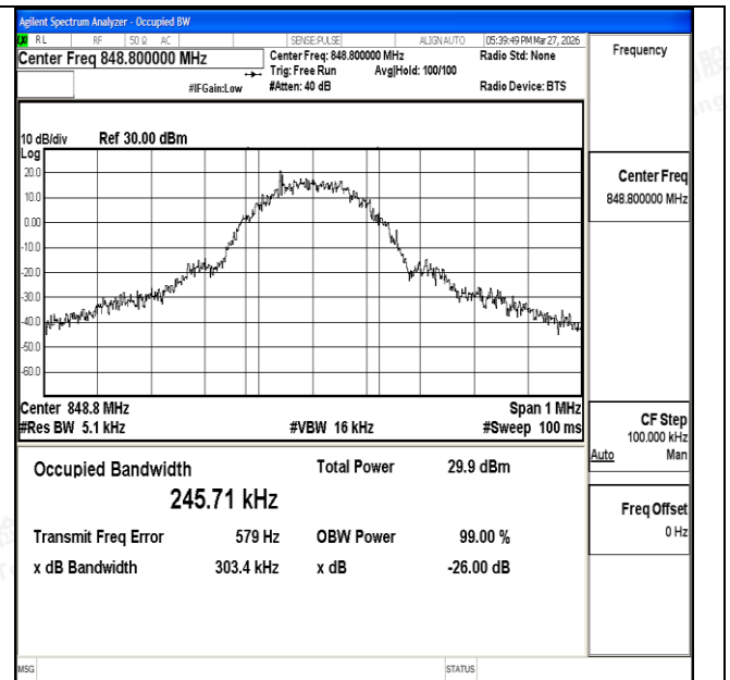
Channel 251 / 848.8 MHz
