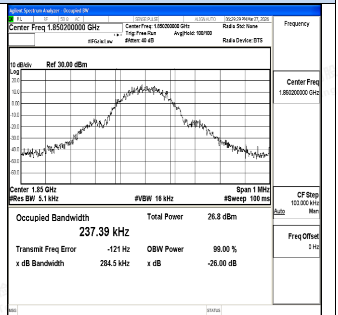
Channel 512 / 1850.2 MHz
