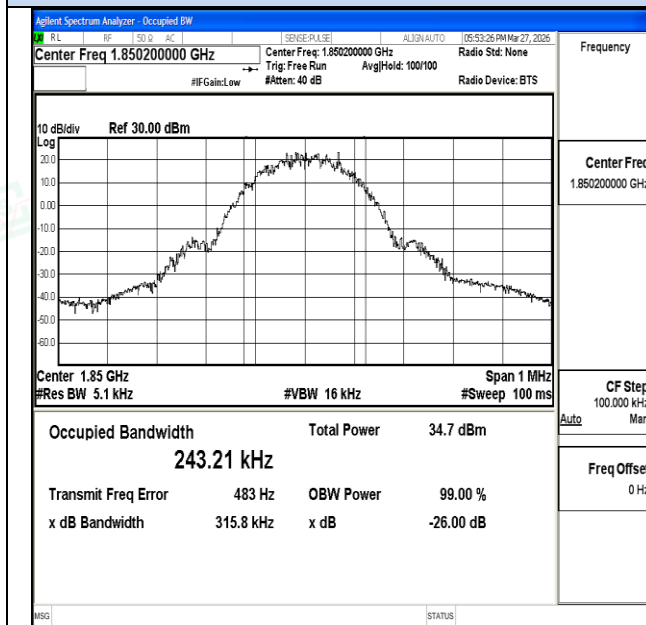
Channel 512 / 1850.2 MHz
