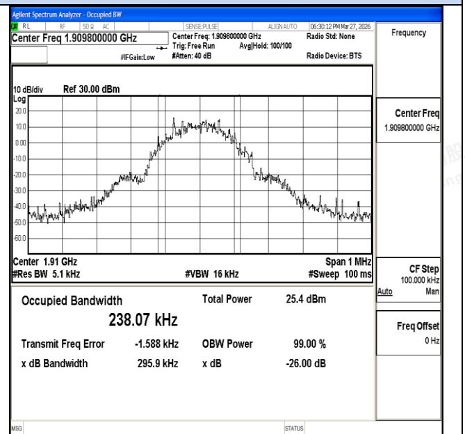
Channel 810 / 1909.8 MHz
