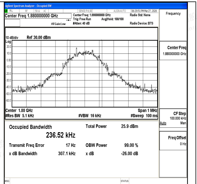
Channel 661 / 1880.0MHz
