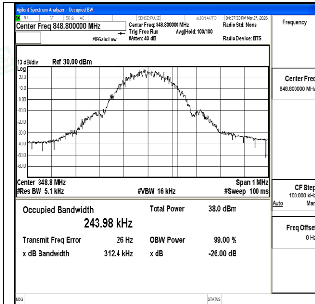
Channel 251 / 848.8 MHz
