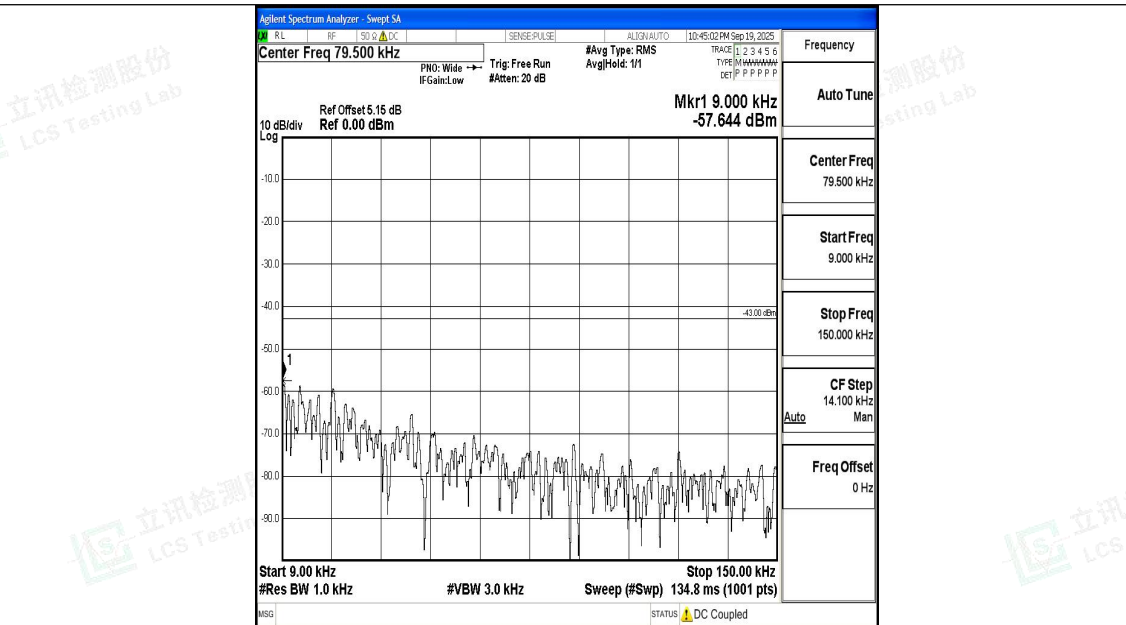
Band2_3MHz_16QAM_19185_1RB#0_0.009~0.15_0.009~0.15
