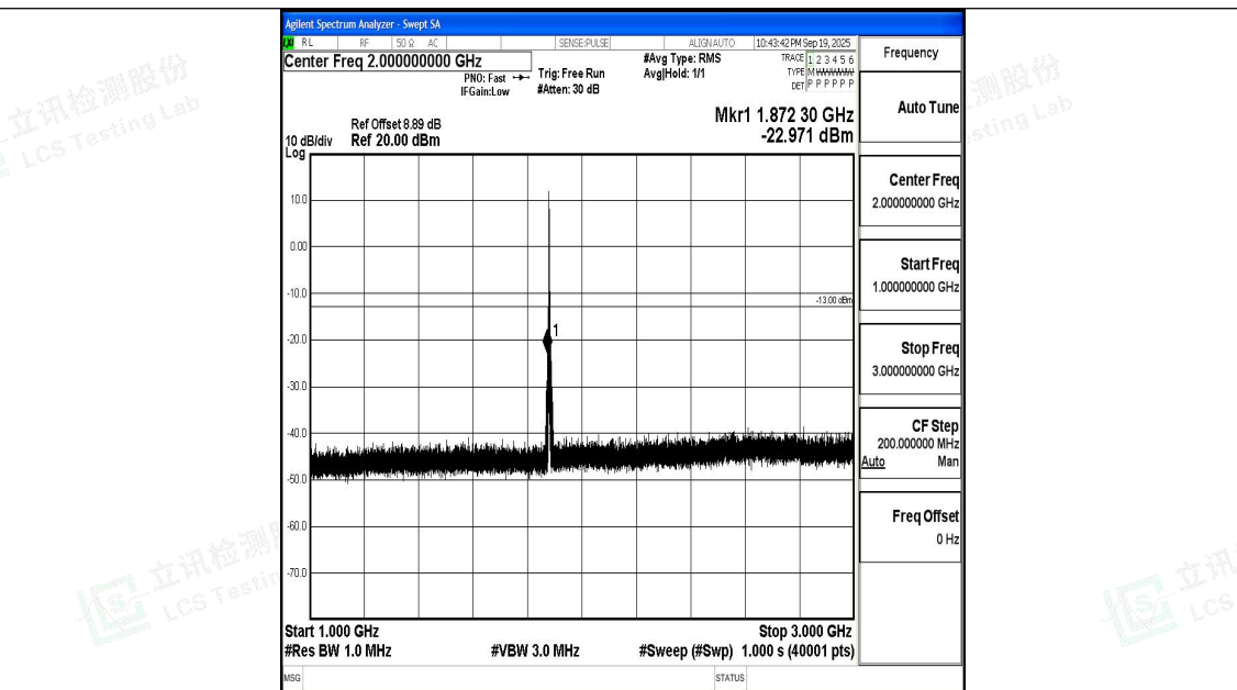
Band2_3MHz_QPSK_18900_1RB#0_1000~3000_1000~3000
