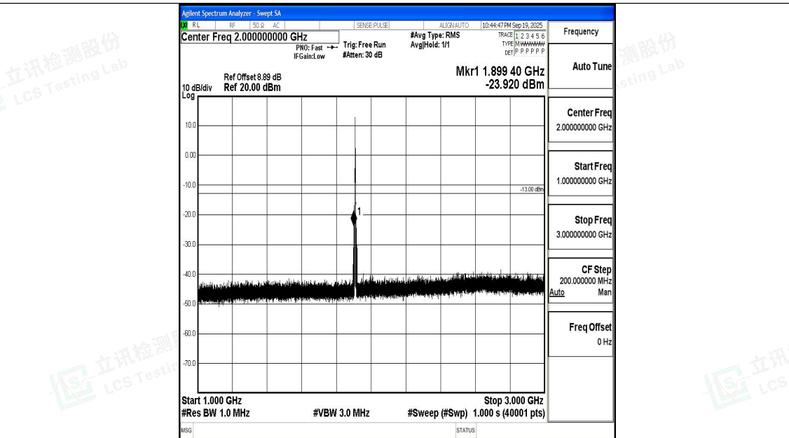
Band2_3MHz_QPSK_19185_1RB#0_1000~3000_1000~3000
