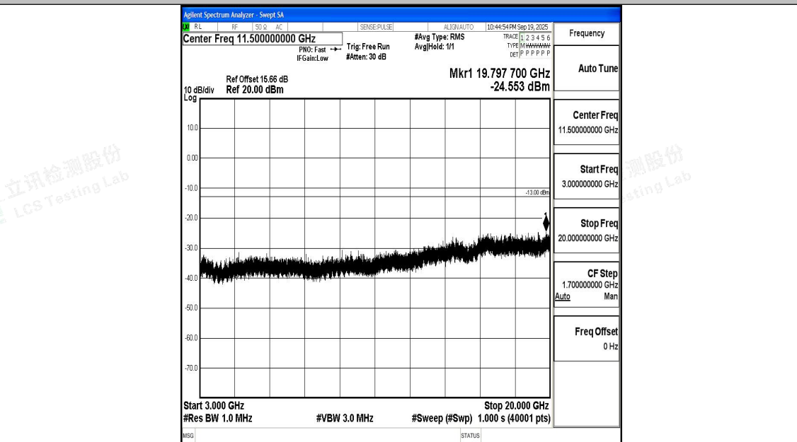
Band2_3MHz_QPSK_19185_1RB#0_3000~20000_3000~20000
