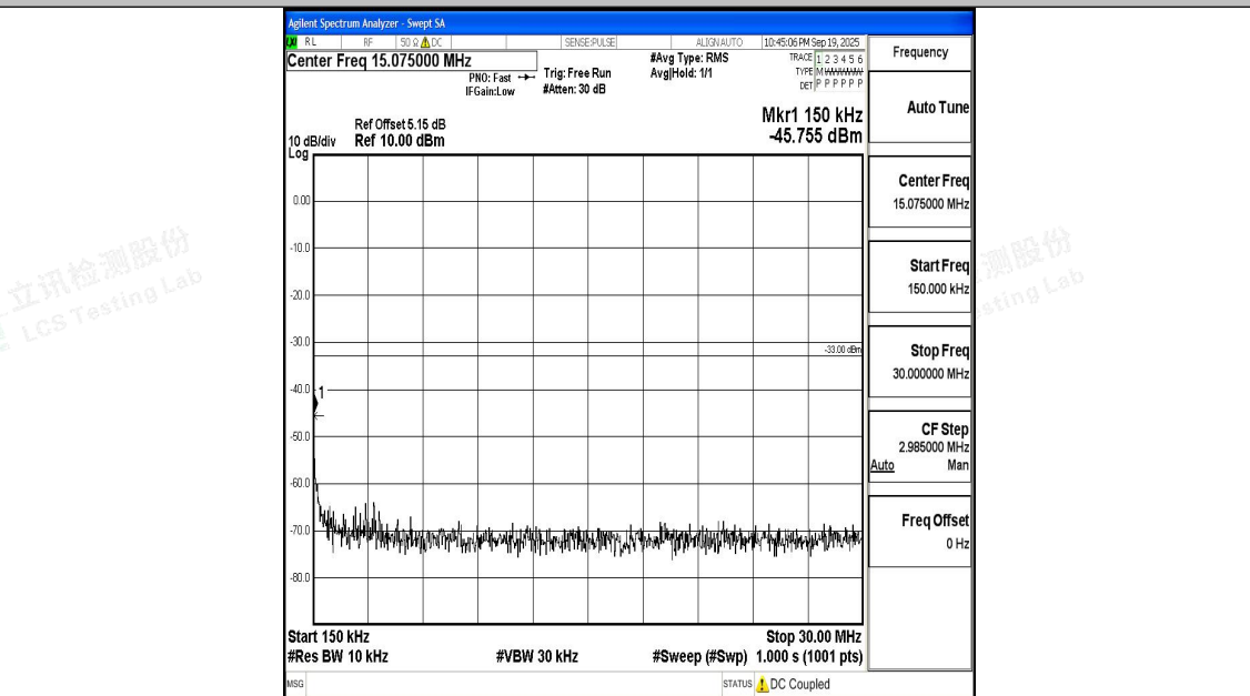
Band2_3MHz_16QAM_19185_1RB#0_0.15~30_0.15~30
